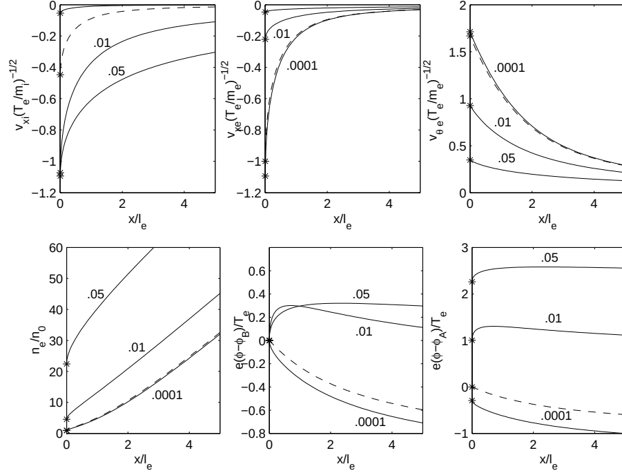
Figure 5: Different plasma profiles for \omega_e/\nu_e = 10 , T_i/T_e = .2 , xenon, and several values of the relative ion backcurrent: solid lines correspond to -I_{iB}/I_d = 0.05, 0.01, \text{ and } 0.0001 ; dashed lines represent the no-sheath case ( -I_{iB}/I_d \simeq 0.009 ). Asterisks correspond to point B.
