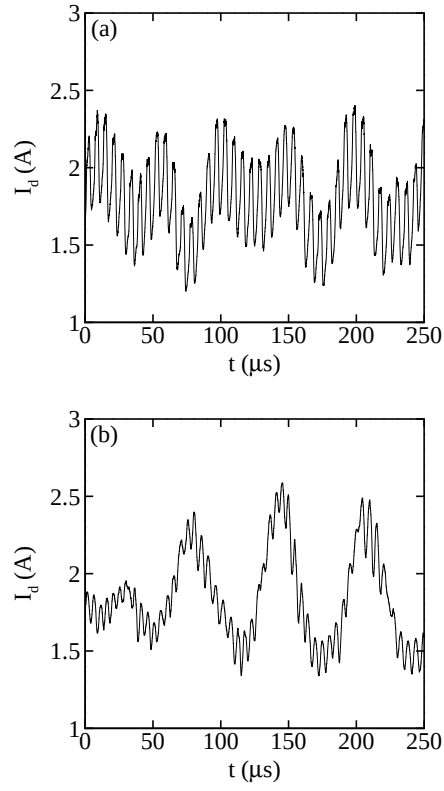
Figure 7: Temporal evolution of the discharge current when (a) the Bohm condition forcing or (b) the corrected weighting algorithm are used by the code.
