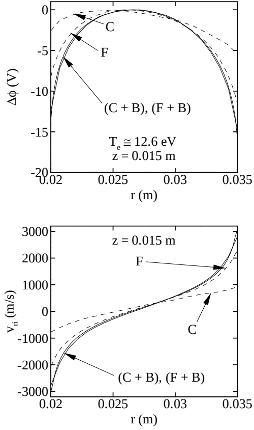
Figure 7: Radial profiles at z = 0.015 m for coarse(C) and fine(F) meshes. (+B) means that Bohm condition forcing is applied.
