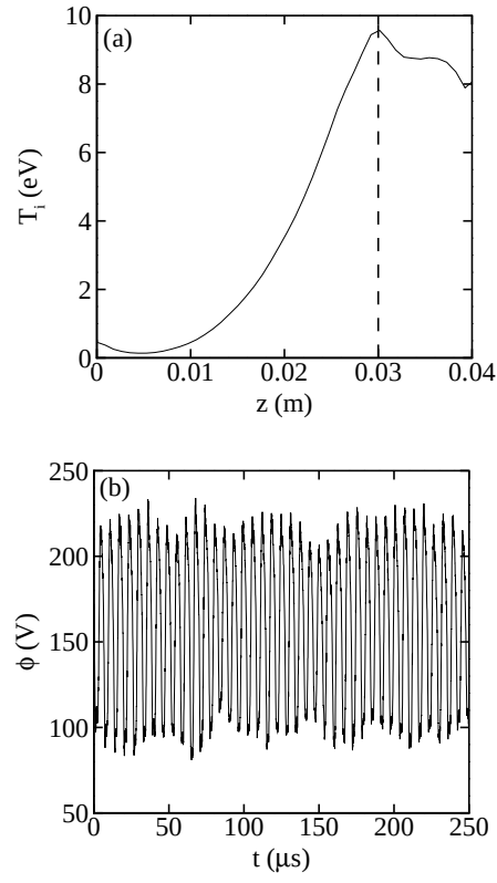
Figure 6: (a) Axial profile of the ion scalar temperature. (b) Temporal behavior of the electric potential at z = 0.03 m and r = 0.0275 m.
