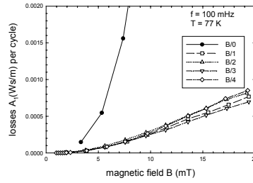
Fig. 3 The hysteresis losses of samples B/0, B/1, B/2, B/3 and B/4 measured at low frequency (100 mHz) and 77 K
