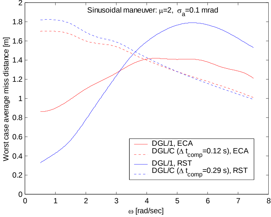
Fig. B.1. Influence of maneuver frequency
