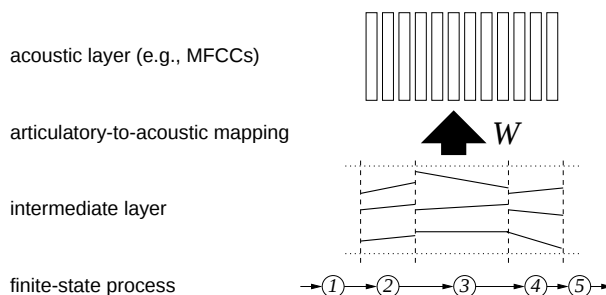
Figure 1: A segmental models that uses linear trajectories in an intermediate space.
