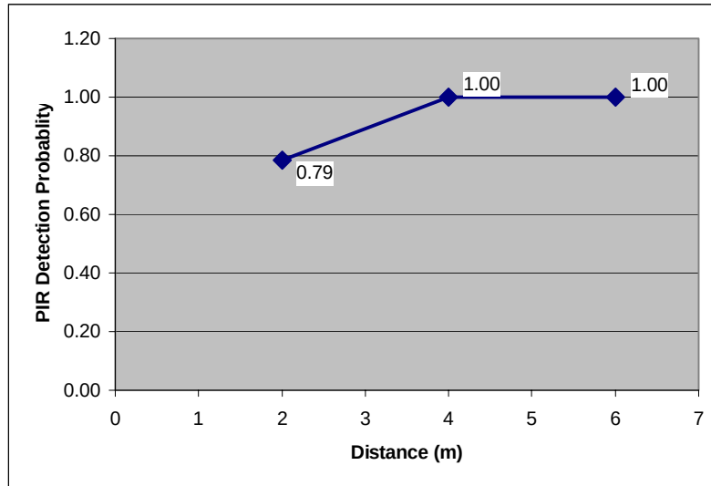
Figure 15. Walking Speed Experiment-1 PIR Detection Probability
