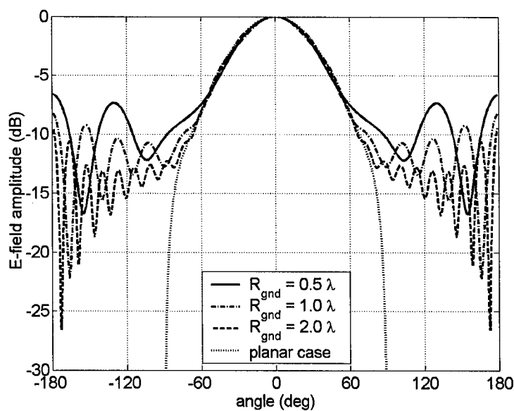
Figure 5.8. Radiation pattern in E -plane of a spherical rectangular patch antenna for different sphere radii.
