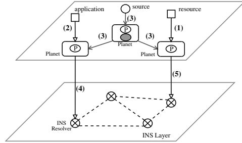
Figure 3. System architecture with both the Solar and INS layers. The shaded circle is an operator that may process events from the source to provide context for an application’s name query or a resource’s name advertisement. The ovals marked with P are proxies representing connected Planet clients. Arrows represent (1) context-sensitive advertisement; (2) context-sensitive query; (3) contextual events; (4) actual query based on current context; (5) actual name advertisement based on current context.
