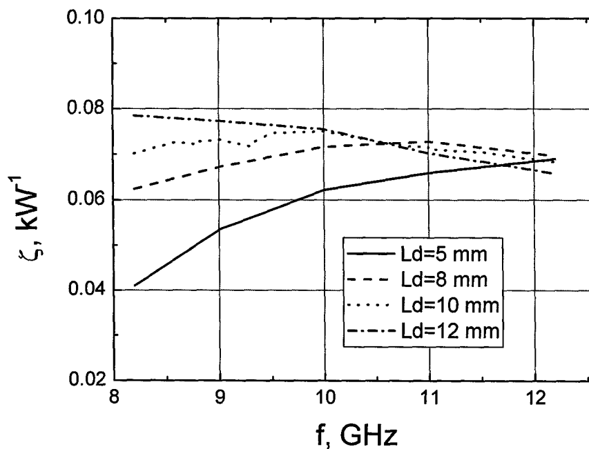
Figure 20. Calculated dependence of the sensitivity in the linear region on frequency for the X-band waveguide-diaphragm-type resistive sensor for different length of the diaphragm: h \times d \times l = 1.0 \times 1.0 \times 1.0 \text{ mm}^3 , \rho = 5 \text{ } \Omega\text{-cm} , Diaphragm length is indicated in the figure.
