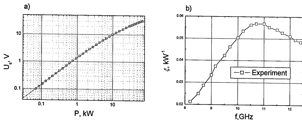
Figure 8. Measured output signal dependence on power at 9.3 GHz using 50 V DC pulse feeding of the RS (a) and the dependence of the sensitivity in the linear region on frequency (b) for typical X-band waveguide-diaphragm-type RS. Electrophysical parameters of the sensor are collected in Table 1.
