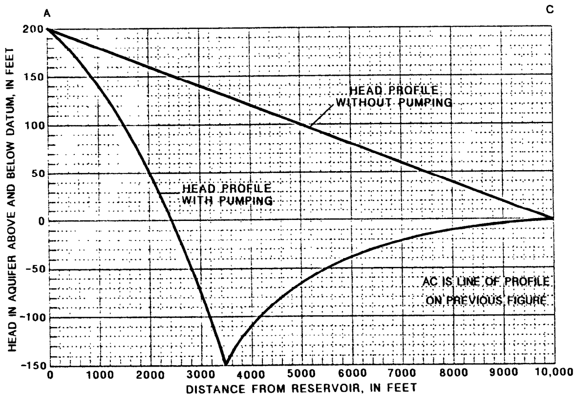
Figure 9-36.--Head profile in the aquifer when the pumping rate of the well is much greater than 3.1 cubic feet per second.
