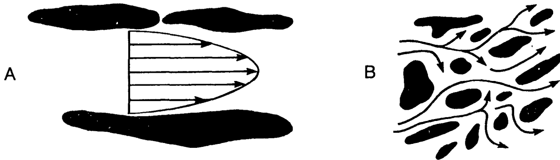
Figure 5-2.--(A) Approximate fluid velocity distribution in a single pore, and (B) tortuous paths of fluid movement in an unconsolidated porous medium.
