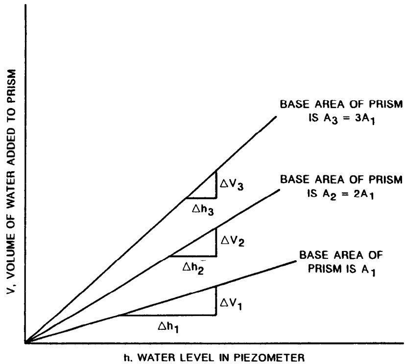
Figure 2-8.--Relation between volume of water injected into a prism of earth material that extends the full thickness of a confined aquifer and head in the prism for different values of prism base area.
