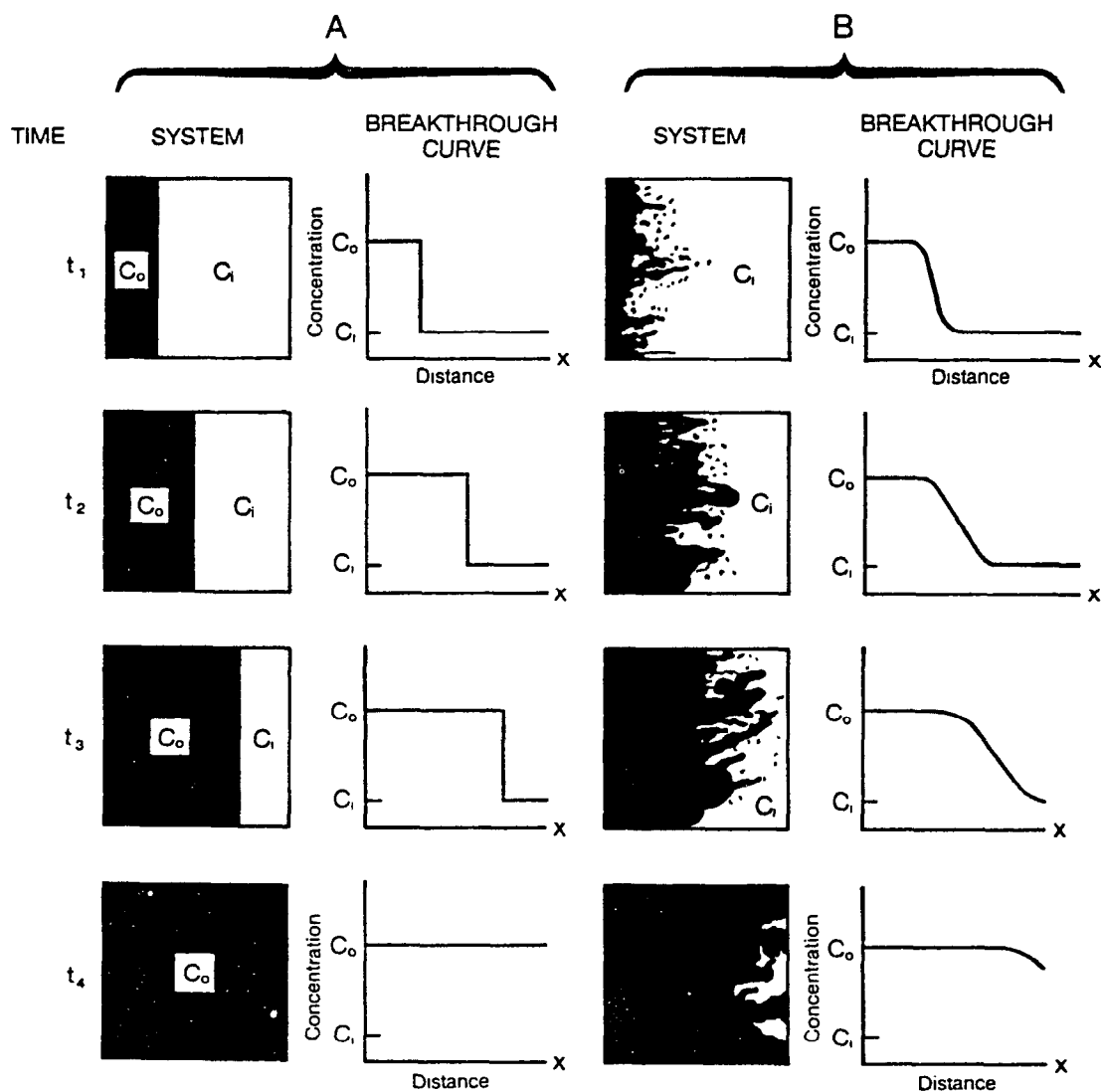
Figure 5-3.--Results of a laboratory experiment to determine the effects of macroscopic heterogeneity on a tracer. (Modified from Skibitzke and Robinson, 1969.)
