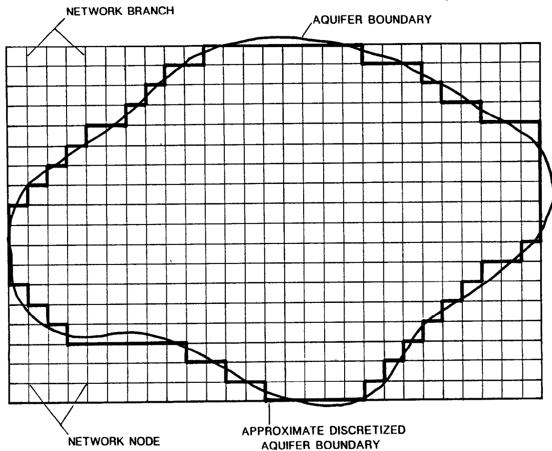
Figure 9-17.--Plan view of a square-mesh finite-difference grid over a map of an aquifer system. (From Prickett and Lonquist, 1971, fig. 7.)
