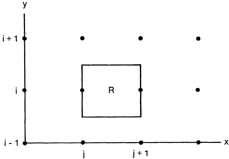
Figure 5-1.--Array of model nodes with region R between two representative nodes (i,j and i,j+1) .
