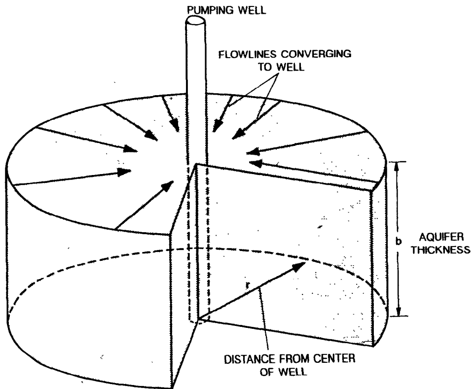
Figure 4-1.--Flow to a well viewed as radial flow through a continuous series of concentric vertical cylindrical sections with the axis of the well at the center.
