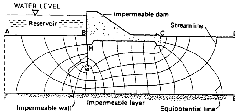
Figure 9-22.--Flow net within three different hydraulic settings: A, through and beneath an earth dam underlain by sloping bedrock; B, beneath a vertical impermeable wall; and C, beneath an impermeable dam and a vertical impermeable wall. (From Franke and others, 1987.)
