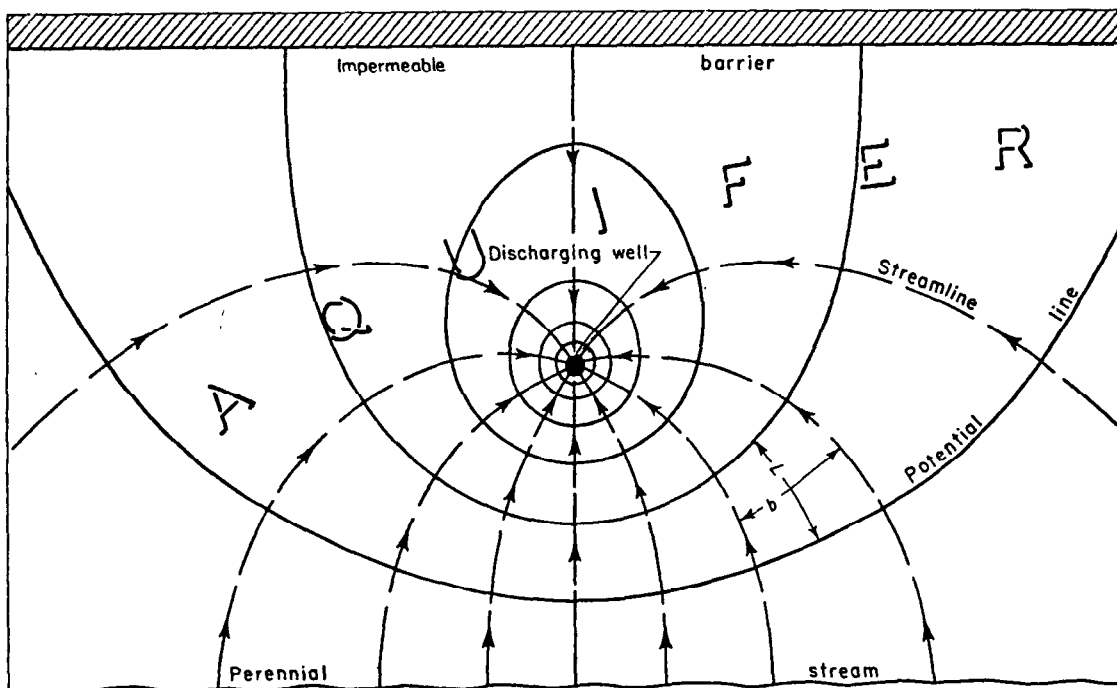
Figure 3-23.--Flow net for a discharging well in an aquifer bounded by a perennial stream parallel to an impermeable barrier. (From Ferris and others, 1962, fig. 9.)
