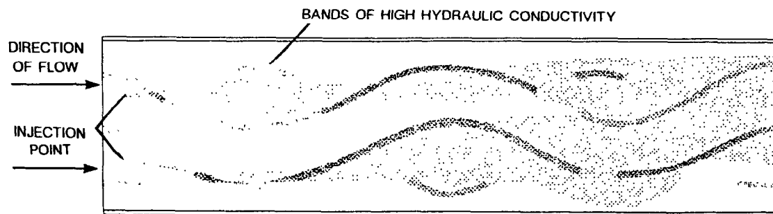
Figure 5-3.--Results of a laboratory experiment to determine the effects of macroscopic heterogeneity on a tracer. (Modified from Skibitzke and Robinson, 1969.)
