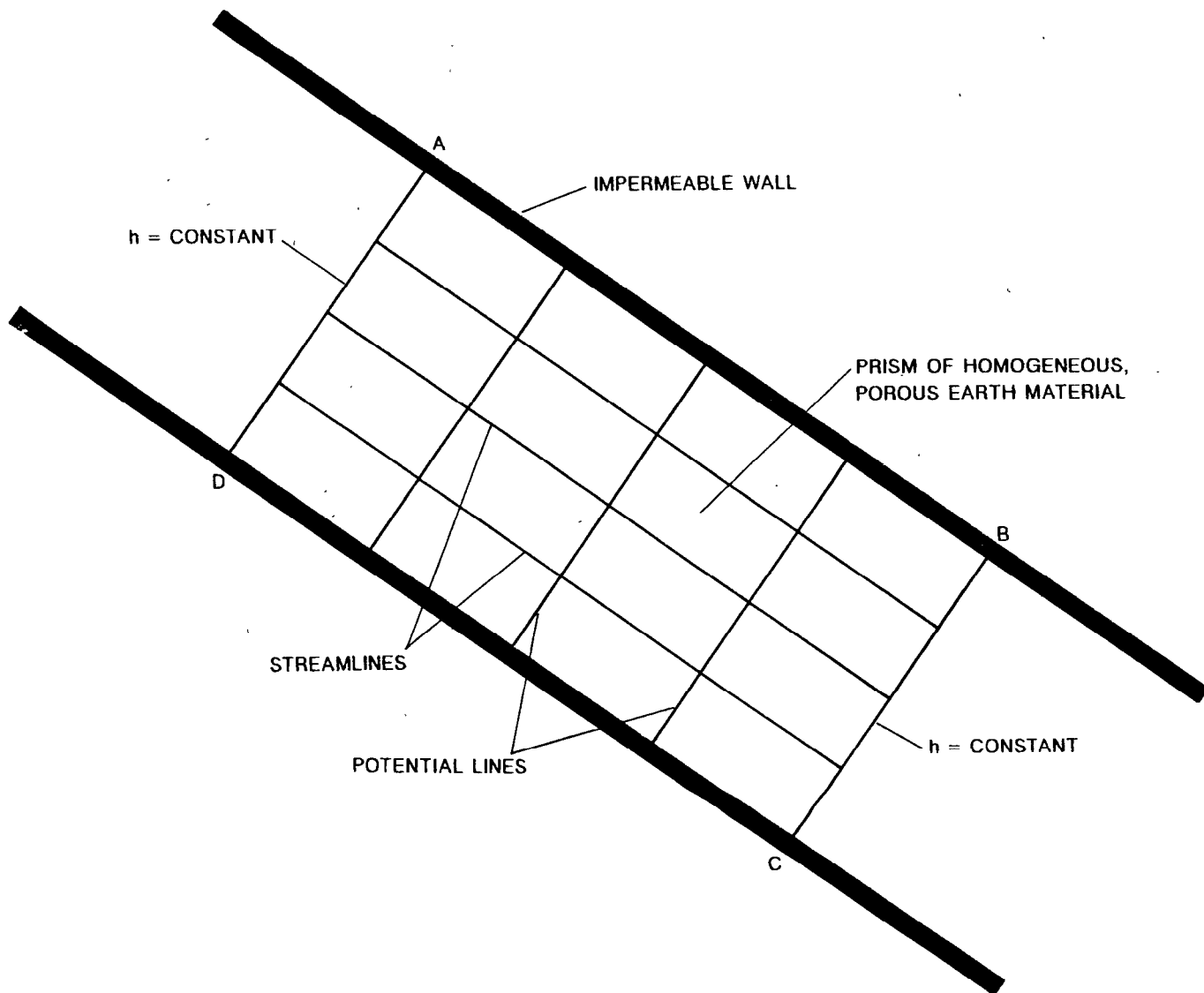
Figure 2-4.--Idealized flow pattern in a Darcy prism, ABCD, composed of homogeneous, porous earth material.
