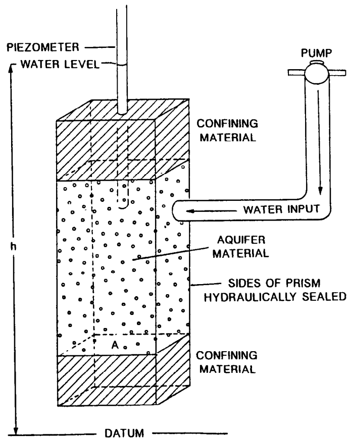
Figure 2-7.--Vertical prism in a confined aquifer bounded above and below by confining material and laterally by walls that are hydraulically sealed. (Modified from Bennett, 1976, p. 55.)
