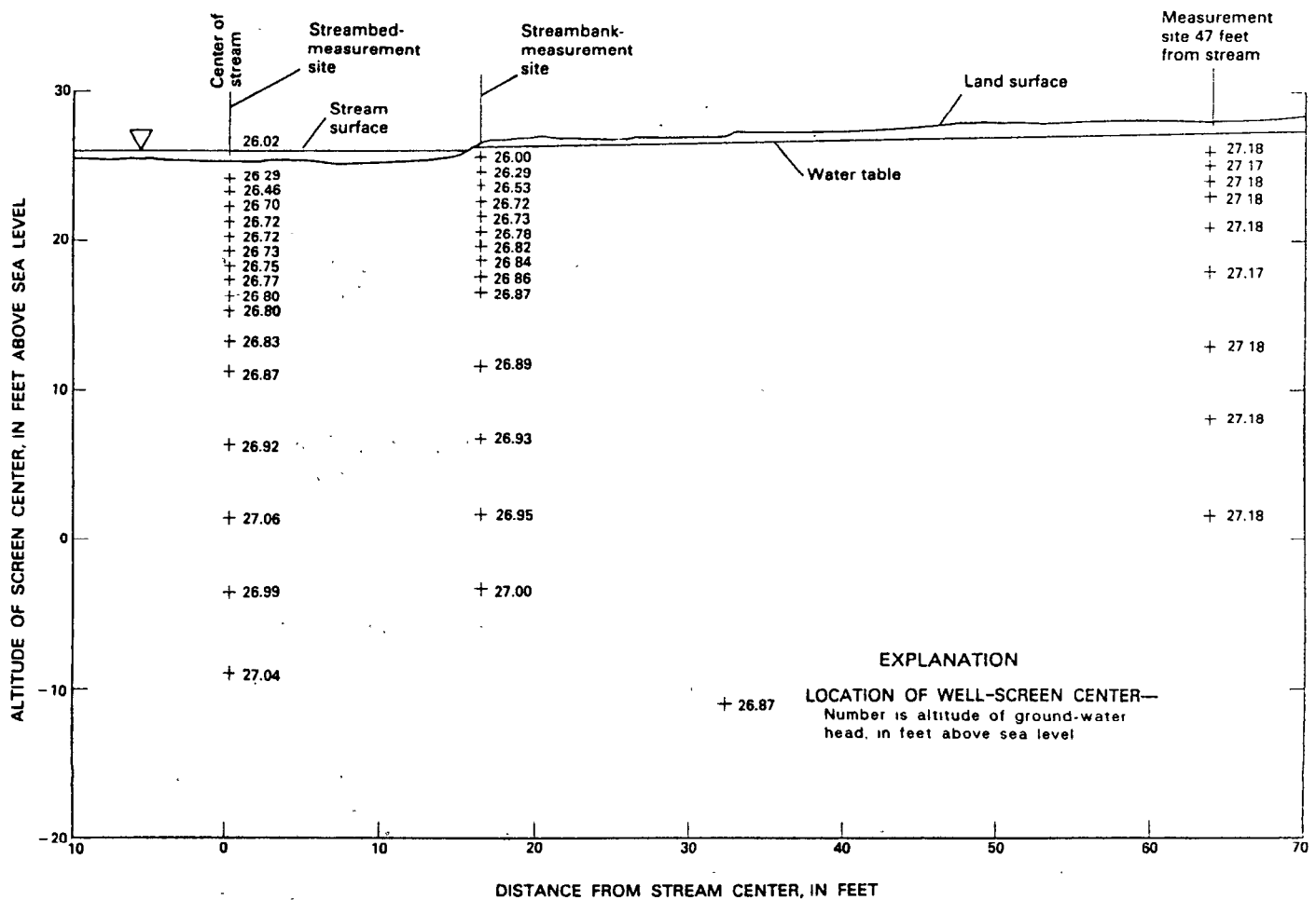
Figure 1-13.--Head measurements near Connetquot Brook, Long Island, New York, during a 3-day period in October 1978. (Modified from Prince and others, 1988, fig. 10.)
