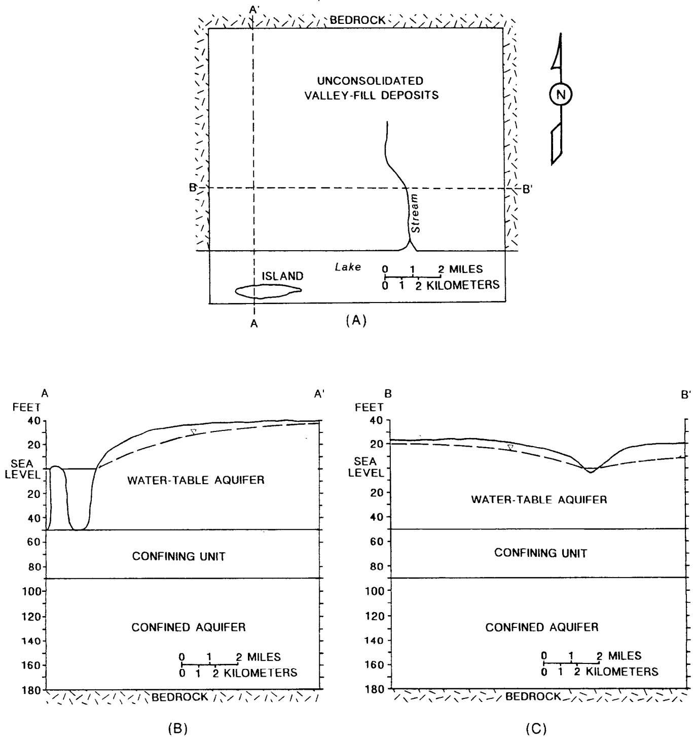
Figure 3-2.--Hydrogeologic framework of hypothetical ground-water system: (A) plan view, (B) north-south-trending section, (C) east-west trending section.
