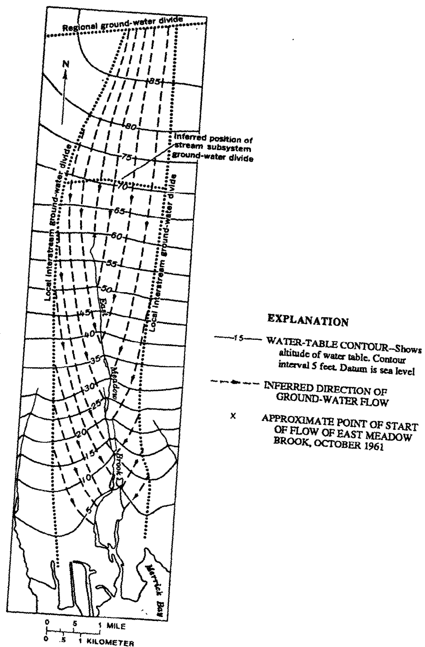
Figure 5-7.--Ground-water flow net in the vicinity of East Meadow Brook, Long Island, New York, in October 1961. (From Franke and Cohen, 1972.)
