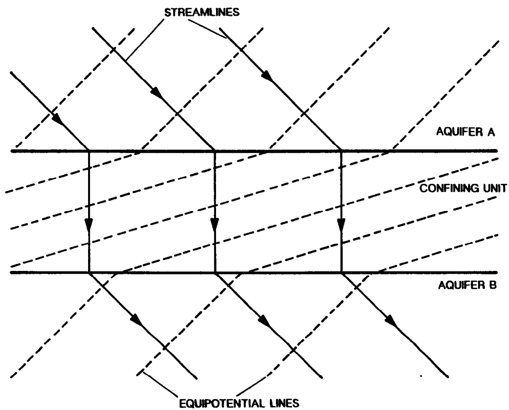
Figure 3-9.--Pattern of streamlines (flowlines) and equipotential lines passing through units with highly contrasting isotropic hydraulic conductivities.
