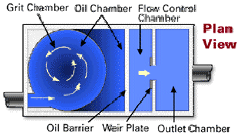
Figure 2. Vortechs' Stormwater Treatment System (Plan View).
