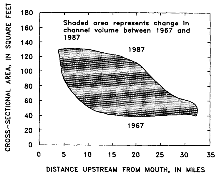
Figure 9.--Idealized example showing determination of change in channel volume using cross-sectional area data.
