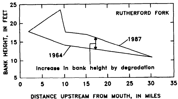
Figure 23.--Changes in bank heights by degradation along the North Fork, South Fork, and Rutherford Fork Obion River, 1964, 1965, and 1987.
