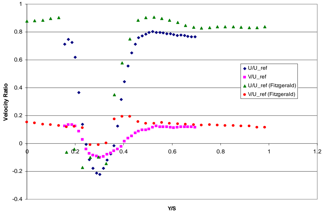
Figure 33. Station 12 survey at Re=666,631
