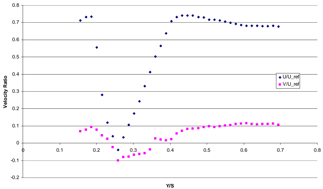
Figure 24. Station 11 survey at Re=467,568
