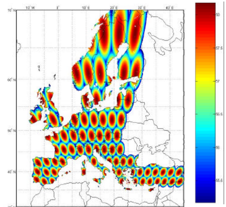
Figure 3: Power radiated by the antenna towards each point of the coverage area in DBi.
