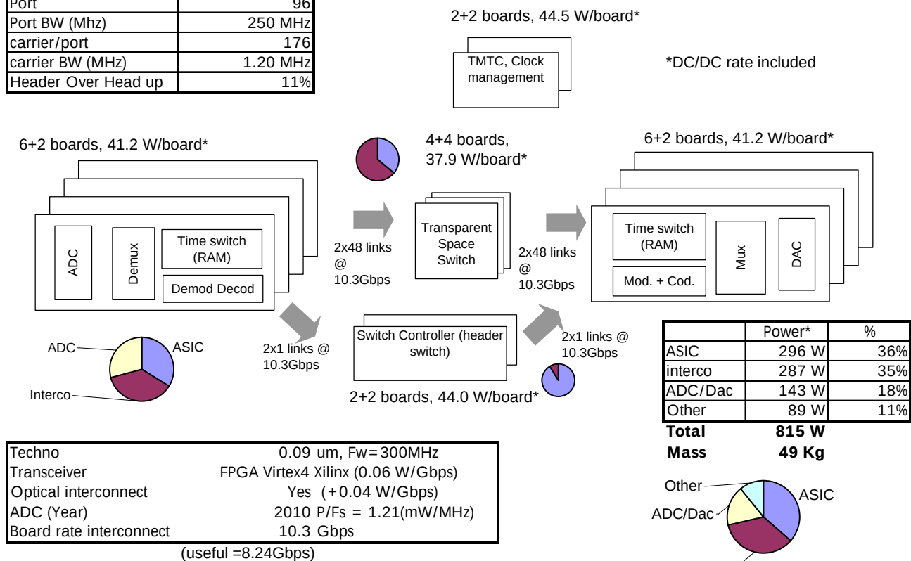
Figure 14 Processor main characteristics at 2010 horizon.
