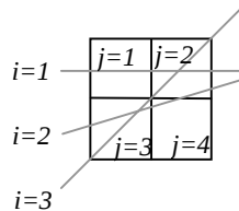
Figure 1. Two-by-two grid with indexed projections, i , and pixels, j .
