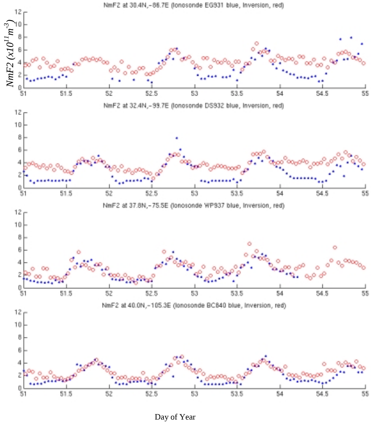
Figure 11. Comparison of NmF2 ( \times 10^{11} \text{ m}^{-3} ) from ionosondes and inversions using ground and space-based GPS data
