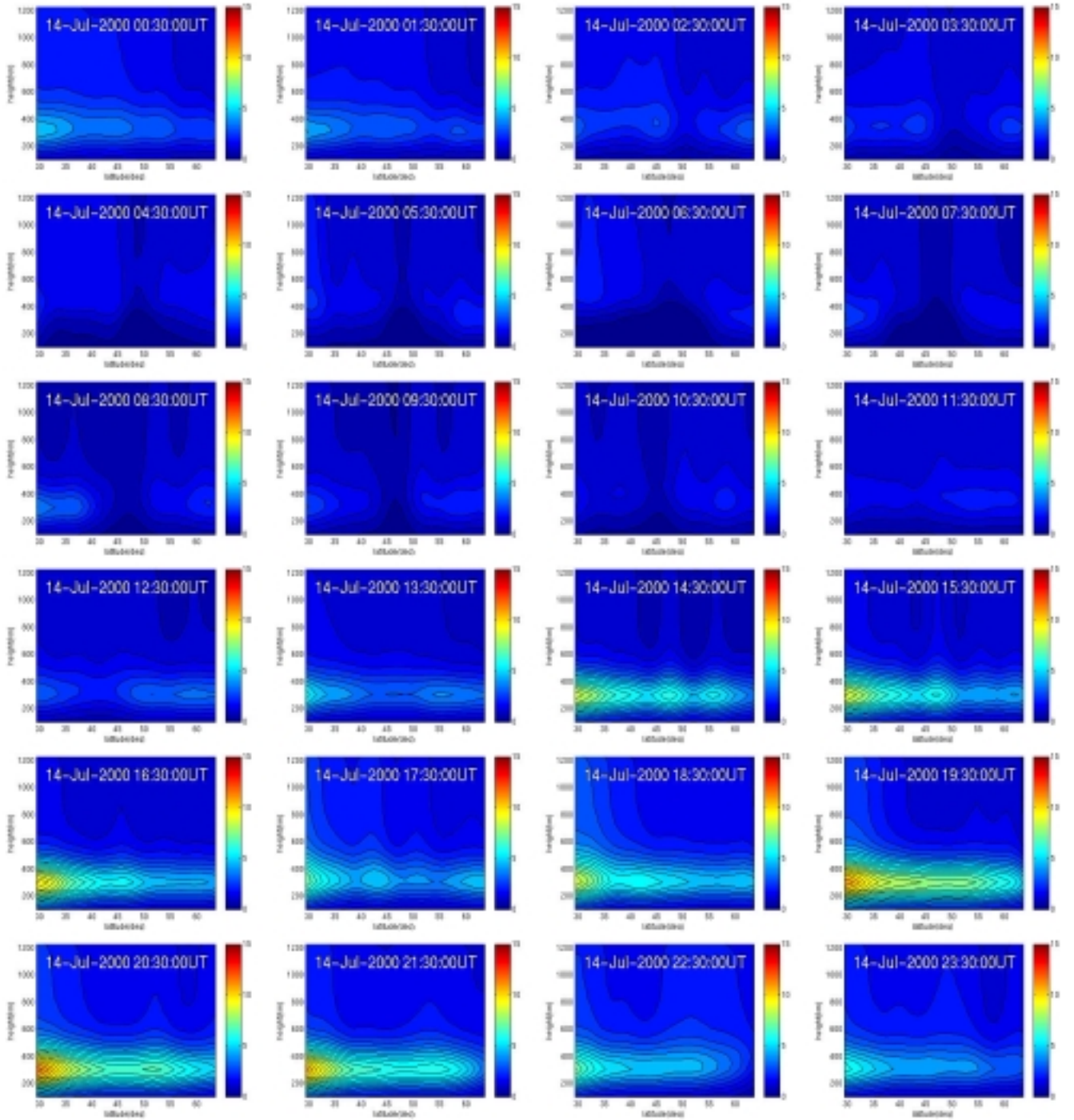
Figure A4. Electron concentration cross-section ( \times 10^{11}/\text{m}^3 ) at 98^\circ\text{W} on 14^{\text{th}} July 2000.
