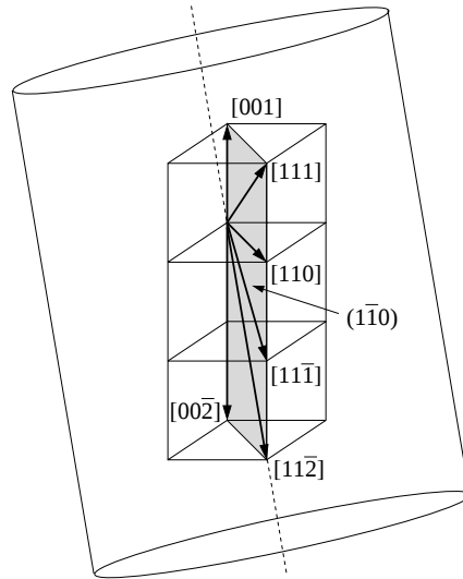
Figure 3. Orientation of Terfenol-D crystals.
