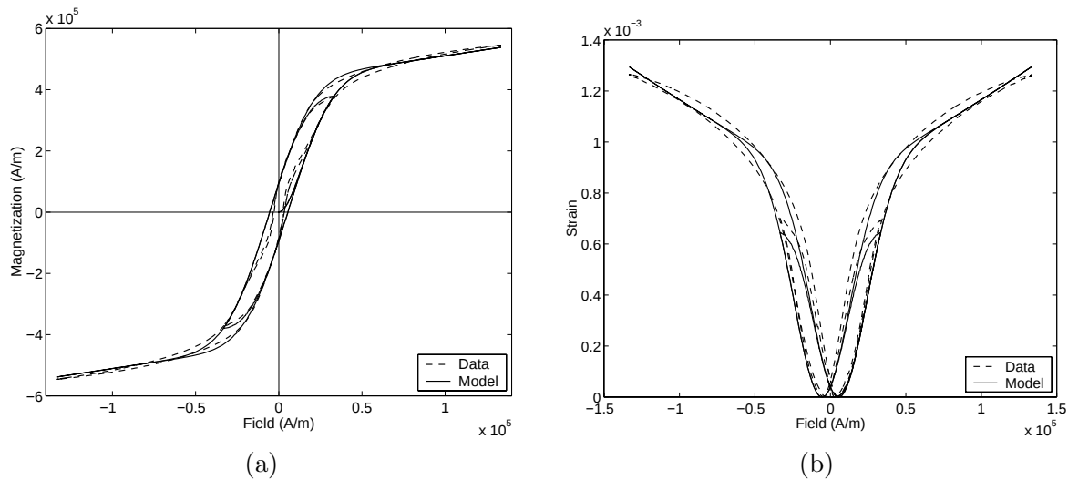
Figure 8. Experimental data (---) from [6] and model response (—): (a) field-magnetization relation, and (b) field-strain relation.
