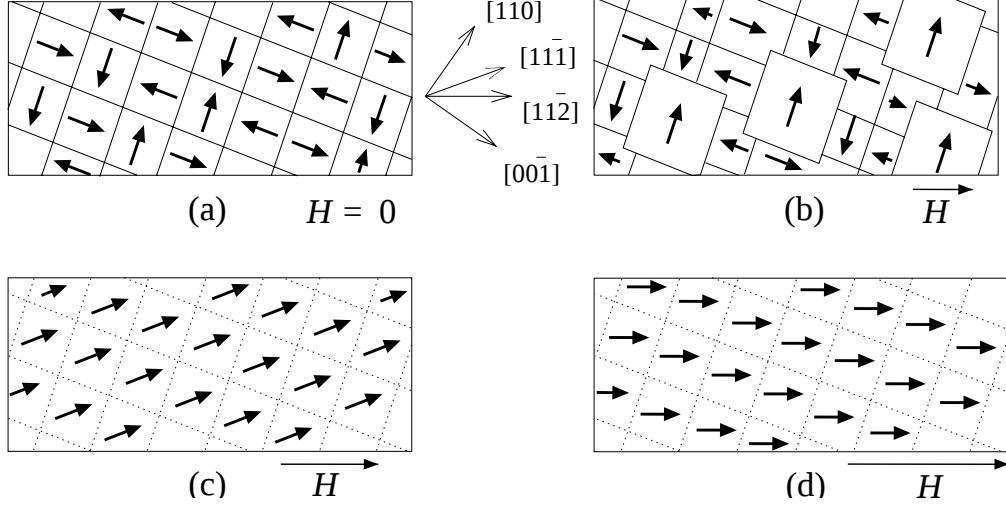
Figure 4. Magnetization process in the (1\bar{1}0) plane of single crystal Terfenol-D due to an applied field H in the [11\bar{2}] direction. (a) Demagnetized state, and (b) growth of domains due to domain wall motion. (c) Rotation of moments to the easy [11\bar{1}] axis, and (d) Rotation of moments to align with the applied field.
