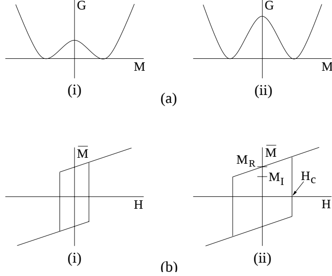
Figure 7. (a) Free energies associated with nonuniform moment distributions. (b) Variations in the local coercive field H_c for the hysteresis kernel due to differing free energies.
