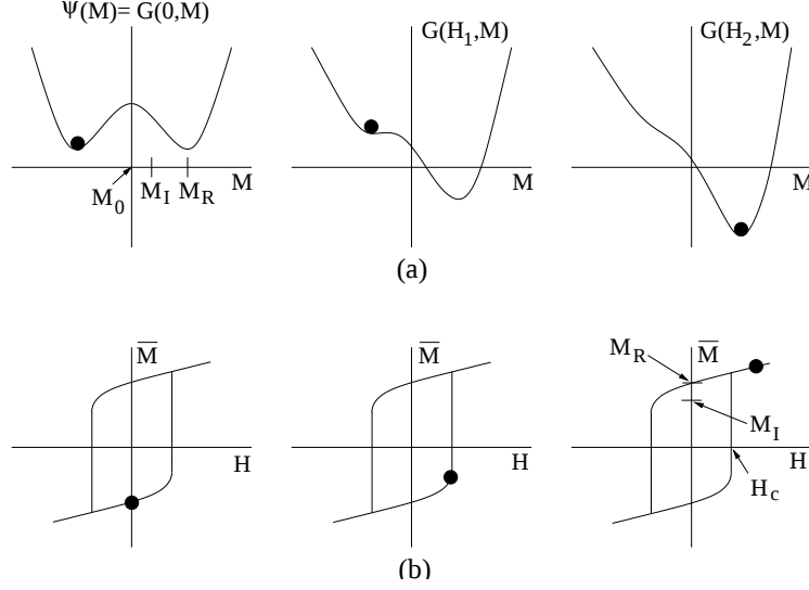
Figure 5. (a) Helmholtz energy \psi and Gibbs energy G for increasing field H ( H_2 > H_1 > 0 ). (b) Local magnetization \bar{M} as a function of H for a homogeneous, isotropic material.
