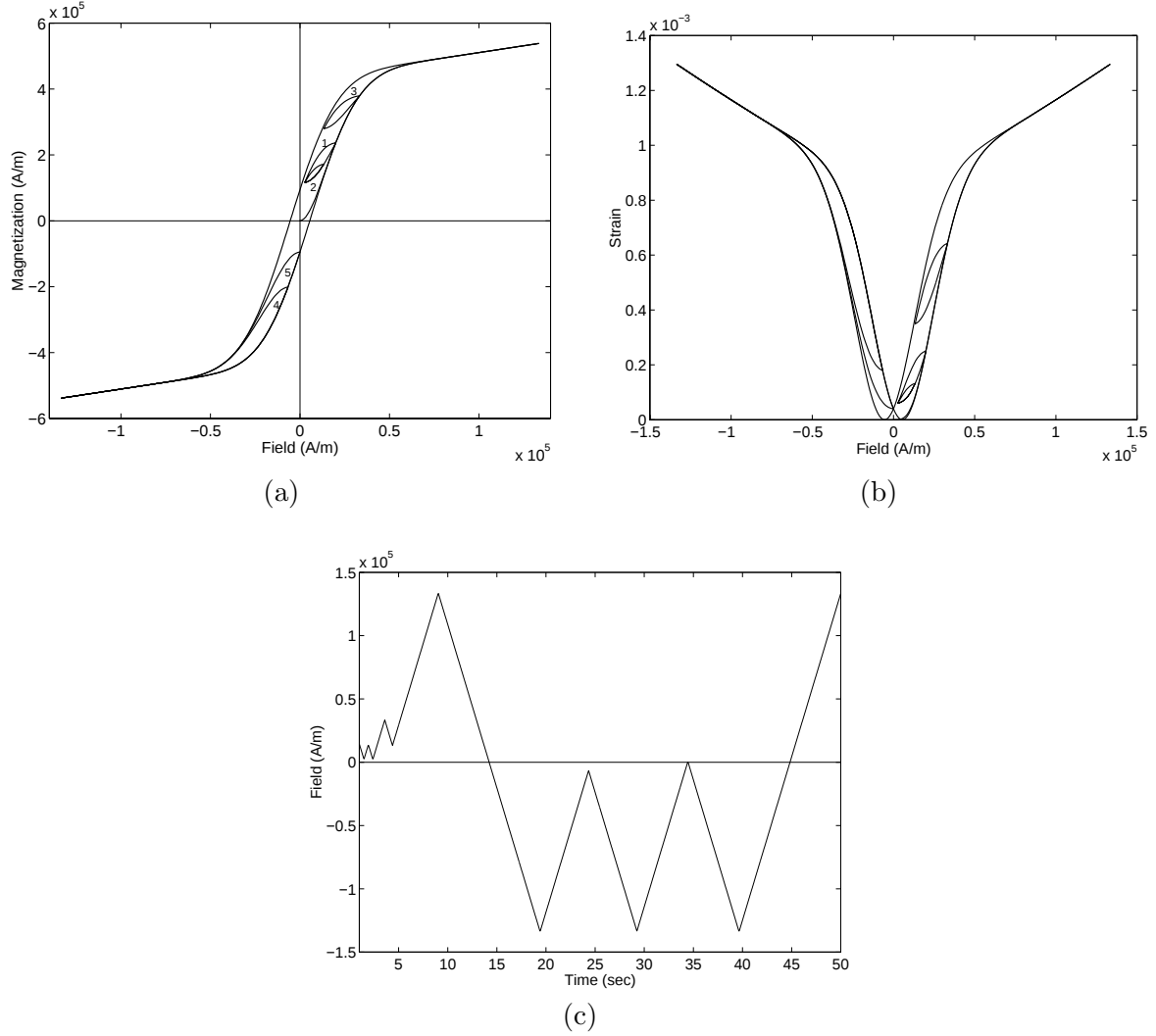
Figure 9. (a) Magnetization predicted by the model, (b) strains profile predicted by the model, and (c) input field H to the model.
