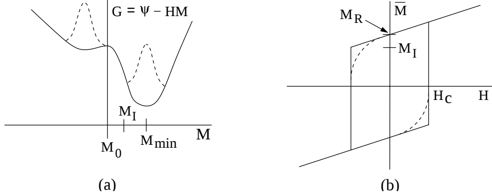
Figure 6. (a) Gibbs energy profile with a high level of thermal activation (---) in the Boltzmann probability \mu(G) = Ce^{-GV/kT} . (b) Local magnetization \bar{M} given by equation (6) with high thermal activation (---) and limiting magnetization \bar{M} specified by (12) in the absence of thermal activation (—).
