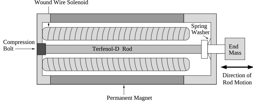
Figure 2. Cross section of a typical Terfenol-D magnetostrictive transducer.
