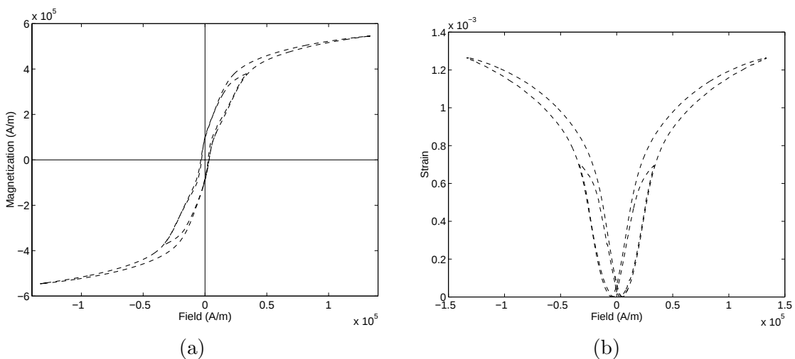
Figure 1. Hysteretic data measured in a Terfenol-D transducer as reported in [6]: (a) field-magnetization relation, and (b) Field-strain relation.
