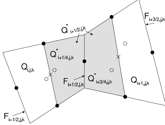
Figure 2: Midsection through two adjoining cells in the logical x direction. Filled and open circles represent locations on faces where fluxes are estimated; open circles represent flux locations on faces in the logical y direction projected onto midsection. The \times symbol is used to denote pressure locations at logical cell centers.
