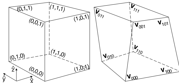
Figure 1: Left: reference cube \hat{Q} with edges of unit length. Right: arbitrary cell Q from discretization with vertex locations \mathbf{v}_{000} , \mathbf{v}_{100} , \mathbf{v}_{010} , \mathbf{v}_{001} , \mathbf{v}_{110} , \mathbf{v}_{101} , \mathbf{v}_{011} and \mathbf{v}_{111} indicated.
