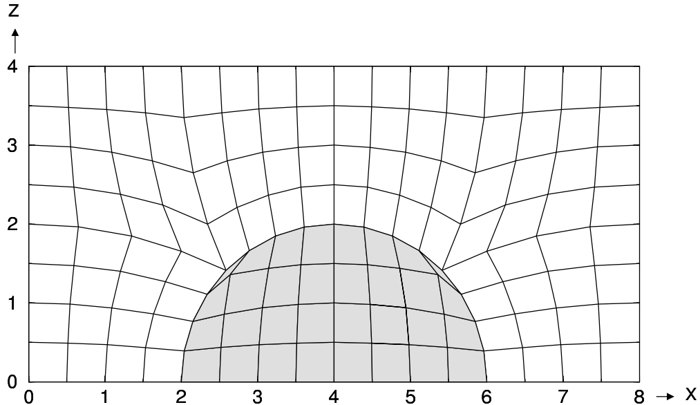
Figure 5: Core discretization for disk-shaped heterogeneity problem. Shaded area represents region of conductivity K_1 ; remaining domain has conductivity K_2 . Flow is largely from left to right.
