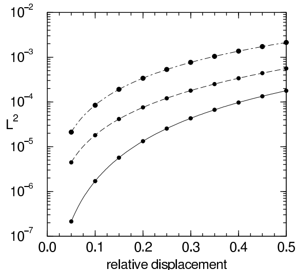
Figure 4: L^2 norm results for various test functions from the uniform flow, simply distorted grid experiment. Solid line: GK test function; dashed line: MCJMR test function; dashed and dotted line: CJMR test function.
