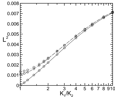
Figure 6: L^2 norm results for various test functions from the 2-D, nonuniform flow experiment. Solid line: GK test function; dashed line: MCJMR test function; dotted line: CJMR test function.
