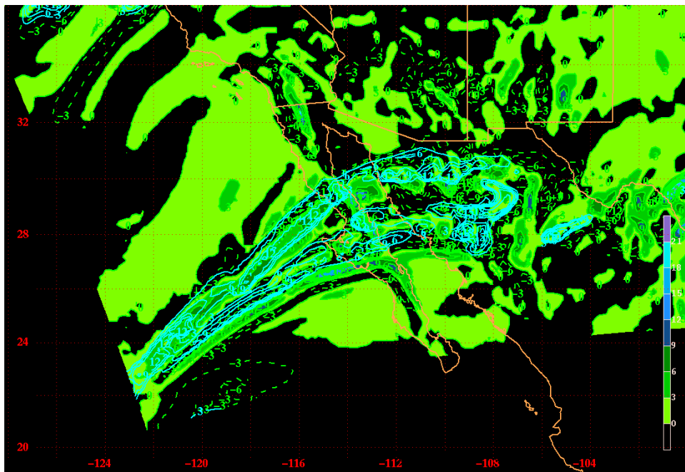
Figure 4.4.a. 2880 sigma ice water mixing ratio and moisture divergence for 21/00Z. Ice water mixing ratio is in grams per kilogram and areas of moisture divergence are shaded.
