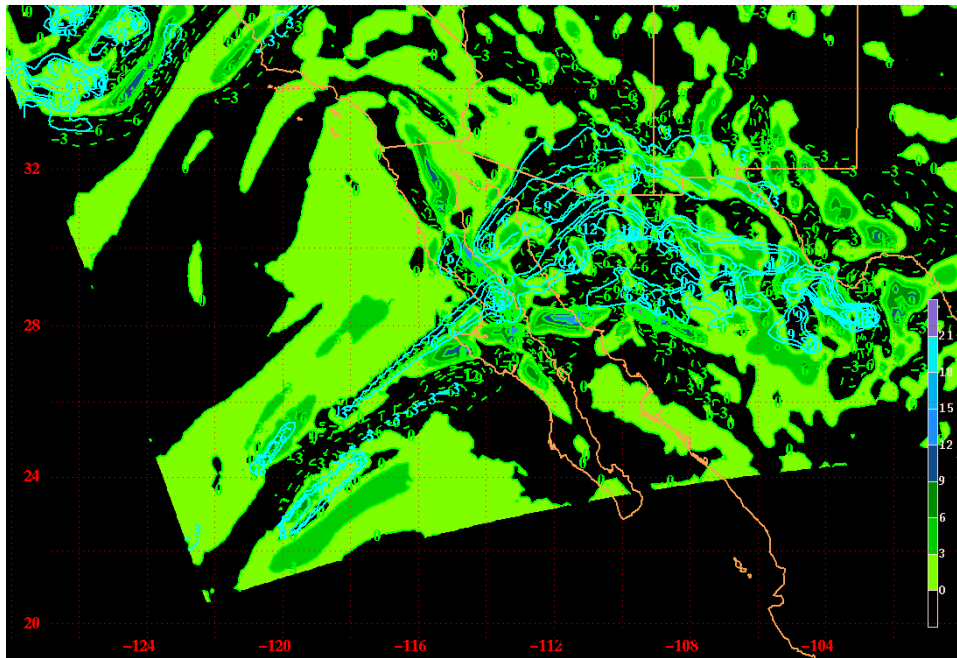
Figure 4.4.d. 2880 sigma ice water mixing ratio and moisture divergence for 21/09Z. Ice water mixing ratio is in grams per kilogram and areas of moisture divergence are shaded.
