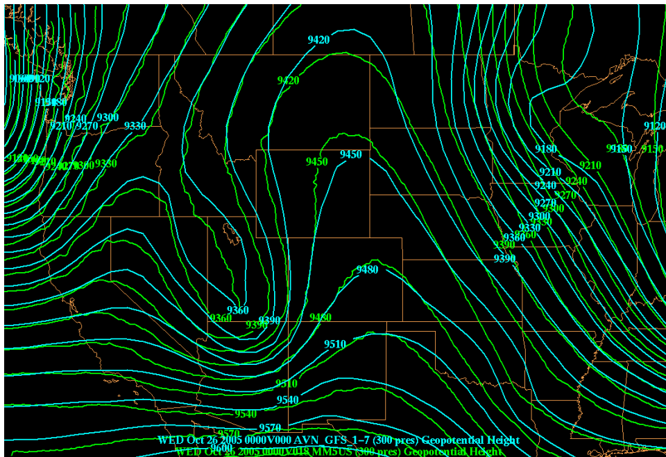
Figure 5.2.a. Verification of the 18-hour MM5 300mb height forecast (green contours) against the corresponding GFS analysis (blue contours) for 00Z on 26 Oct 05.
