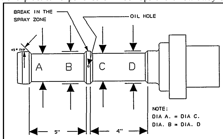
Figure 6.8 UNDERCUT DESIGN FOR OIL HOLE (Interrupted Spray Zone)
