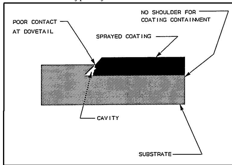
Figure 6.3 POORLY DESIGNED UNDERCUT
