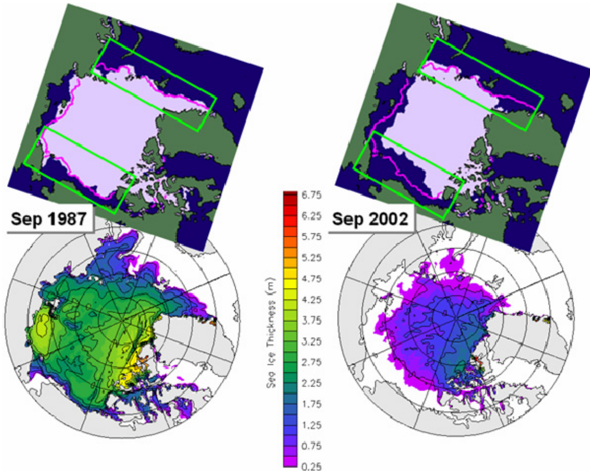
Figure 32. Summer 1987 and 2002 Arctic ice extent and distribution. The upper plots show SSM/I ice extent, the lower ones NPS model output ice thickness distribution. Areas with ice concentrations less than 15% are excluded. The pink line in the upper plots represents mean ice extent for this time of year. [After Maslowski 2006]
