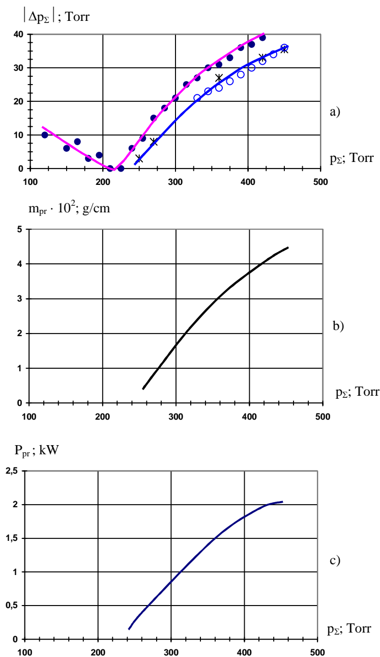
Fig.6.1.1. Dependence on initial pressure in the tank with propane: a) – of the pressure change during time of the valve switch on, б) – of the average mass flux of propane, c) – of burning power of propane in supposition of its full oxidation.
