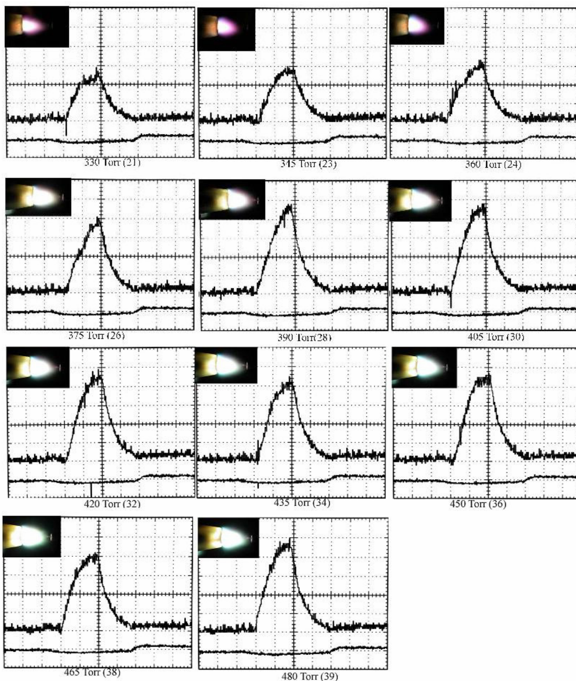
Fig.6.5.1. Waveforms of the temperature gauge at different magnitudes of initial pressure in the propane tank
