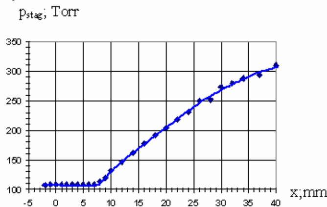
Fig.6.3.3.a. Measured dependence p_{stag}(x)
