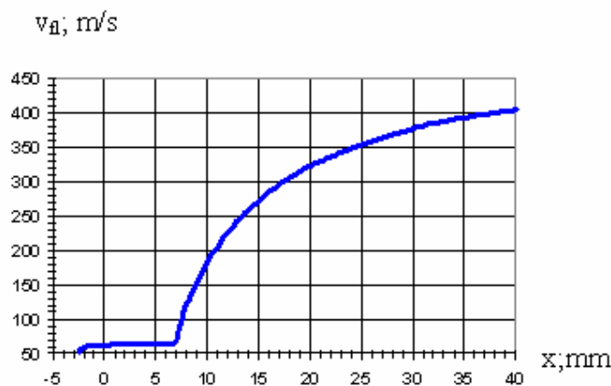
Fig.6.3.3b. Dependence v_{fl}(x) , calculated from Fig.6.3.3a
