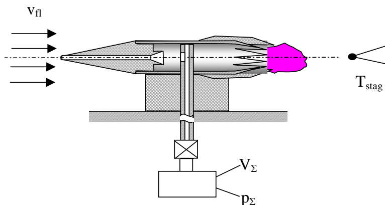
Fig.6.1. Sketch of device for ignition of air-propane mix by attached undercritical MW discharge in SS flow
