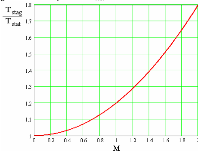
Fig.3.13 Graph of stagnation temperature and static temperature ratio via Mach number ( \gamma = 1.4 ).
