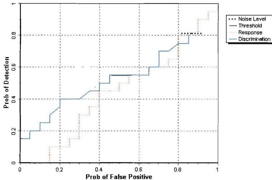
Figure 2. GEM-3 Realtime Disc/hand held blind grid probability of detection for response and discrimination stages versus their respective probability of false positive over all ordnance categories combined.
