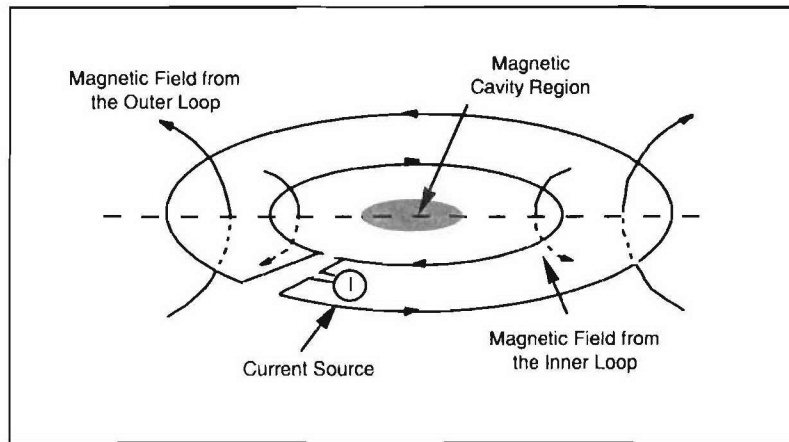
Figure 2. Conceptual representation of the GEM-3 coils.
