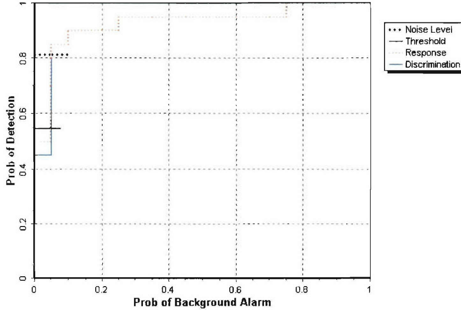
Figure 3. GEM-3 Realtime Disc/hand held blind grid probability of detection for response and discrimination stages versus their respective probability of background alarm over all ordnance categories combined.
