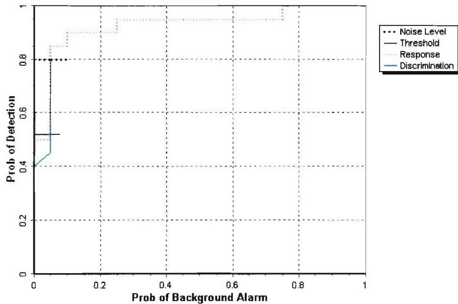
Figure 5. GEM-3 Realtime Disc/hand held blind grid probability of detection for response and discrimination stages versus their respective probabilities of background alarm for all ordnance larger than 20 mm.
