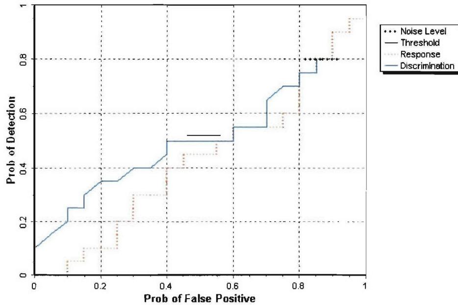
Figure 4. GEM-3 Realtime Disc/hand held blind grid probability of detection for response and discrimination stages versus their respective probability of false positive for all ordnance larger than 20 mm.
