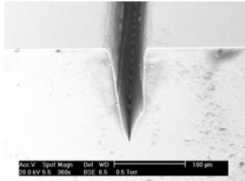
Figure 3.9(a) Trench created using 128 passes at 20μJ
