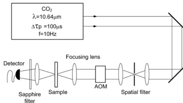
Figure 6.1 schematic of \text{CO}_2 laser test.
