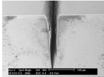
Figure 3.9(b) Trench created using 256 passes at 20μJ
