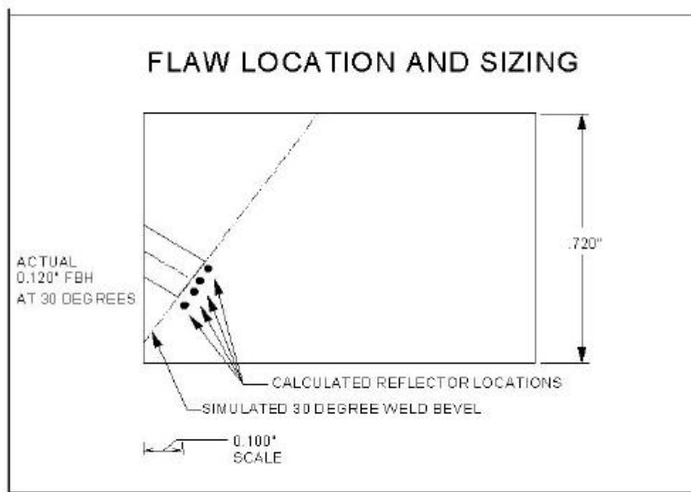
Figure 6 - 3 mm Flat Bottomed Hole Indication
