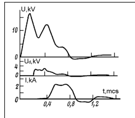
Fig.2.5. Waveforms of the discharge voltage U , at the probe U_z and current I at U_0 = 17 kV and C_0 = 15 nF [10].
