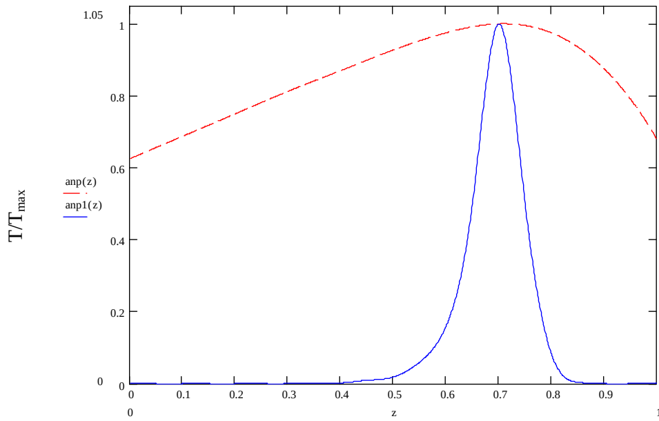
Fig.3.6. Normalized temperature T_0 (dashed curve) and the charge concentration (solid curve) distributions over the boundary layer cross section. ( T_{\max}=2700 K, n_{e\max}=5 \cdot 10^{10} \text{ cm}^{-3} ).
