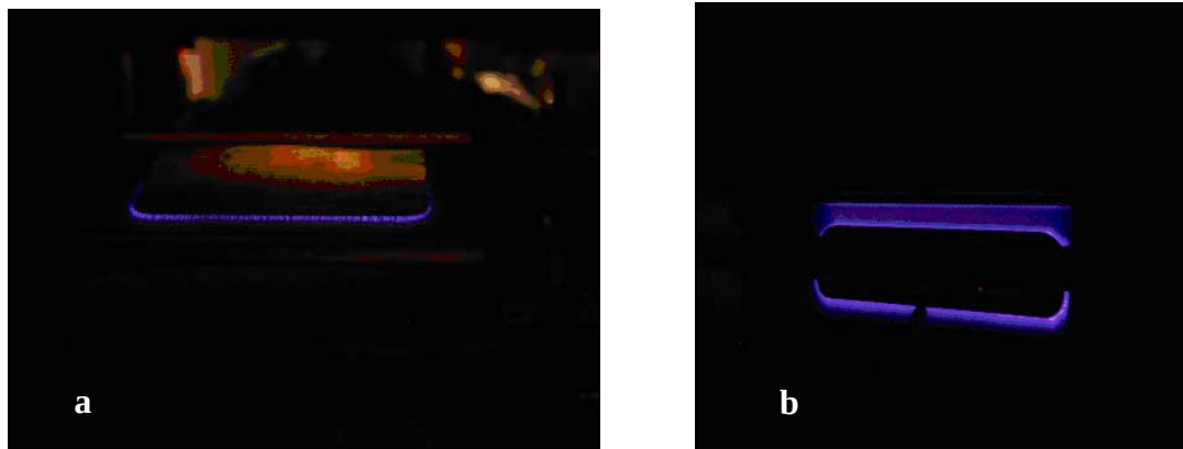
Fig.1.15. Sliding discharge for aerodynamics experiments.
