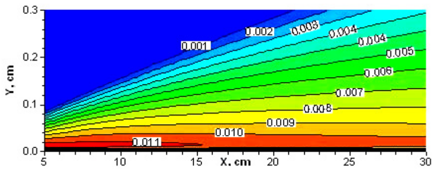
(a) Turbulent energy t = 0 \mu s
