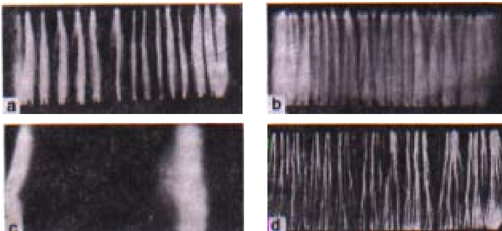
Fig.2.9. Photos of sliding discharge plasma integral luminescence at L \times H = 4 \times 10 \text{ cm}^2 and d = 6 \text{ mm} : a – He, \epsilon \approx 4 ; b – He, \epsilon \approx 250 ; c – air, \epsilon \approx 4 ; d – air, \epsilon \approx 250 .
