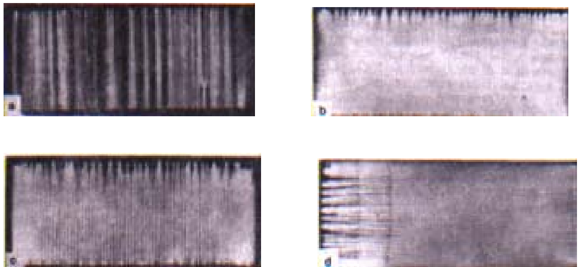
Fig.2.11. Photos of sliding discharge plasma integral luminescence at U_0=50 kV \varepsilon \approx 4 : a –air, d=0.4 mm, L=4 cm; b - He , d=1 mm, L=4 cm; c - He, d=0.4 mm, L=4 cm; d - He, d=1 mm, L=10 cm.
