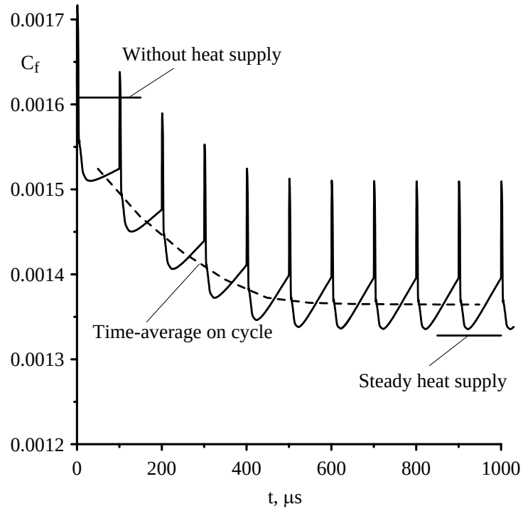
Fig.4.29. Time variation of total skin-friction coefficients for M_\infty = 3.0
