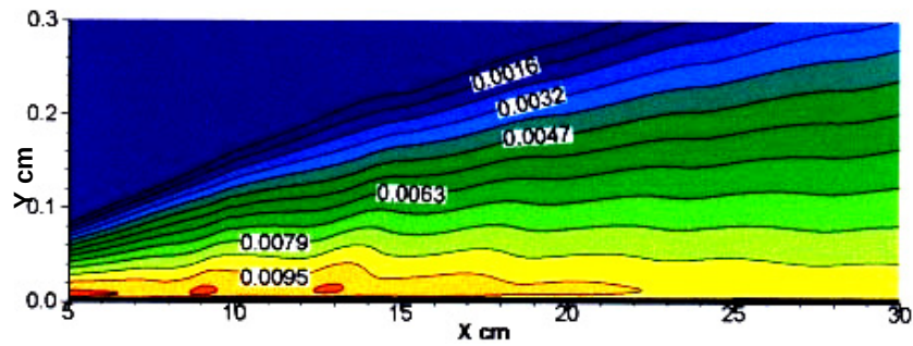
(c) Turbulent energy, t = 801 \mu s
