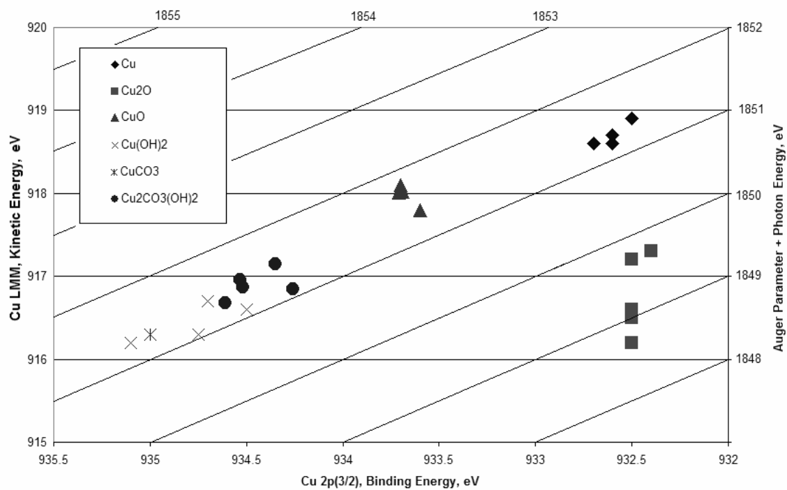
Figure I.5 Chemical State Plot: Malachite [Cu 2 CO 3 (OH) 2 ] with other Referenced Copper Species
