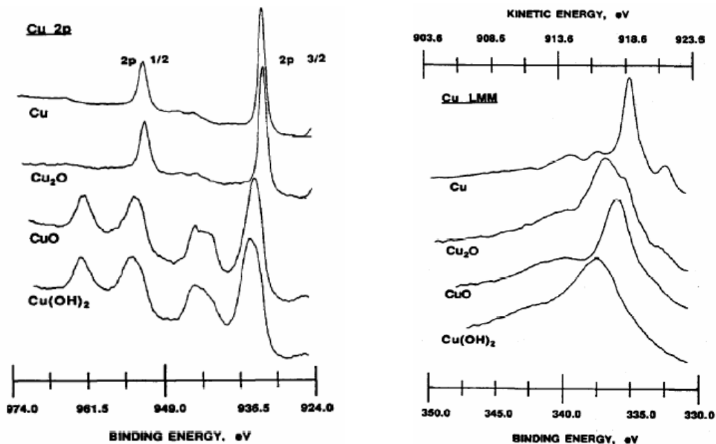
Figure 4.8 Montage of Copper Oxide Spectra (Chawla et al., 1992)
