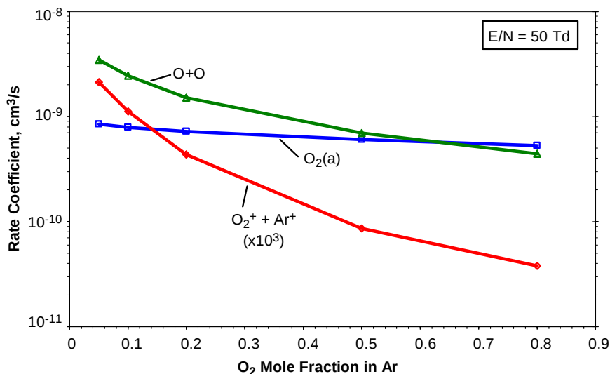
Figure 5: Effect of variations in \text{O}_2 mole fraction on computed electron-impact rate coefficients for \text{O}_2(\text{a}) excitation, \text{O}_2 dissociation, and total ionization for discharge-excited \text{O}_2/\text{Ar} mixtures, E/N = 50 \text{ Td} .
