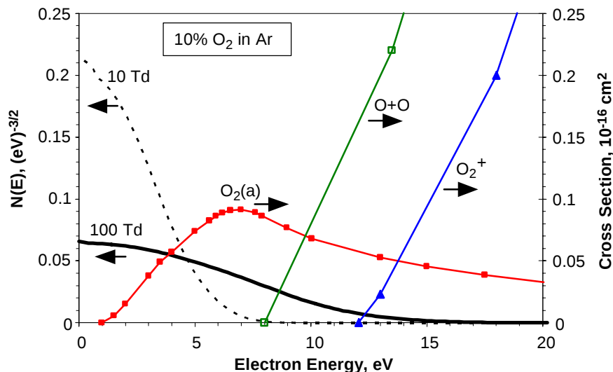
Figure 4: Illustration of overlap of electron energy distributions with electron impact excitation cross sections for \text{O}_2(\text{a}) excitation, \text{O}_2 dissociation to form \text{O} + \text{O} , and \text{O}_2 ionization to form \text{O}_2^+ . The electron energy distributions are computed for E/N = 10 and 100 \text{ Td} , in 10% \text{O}_2/\text{Ar} .
