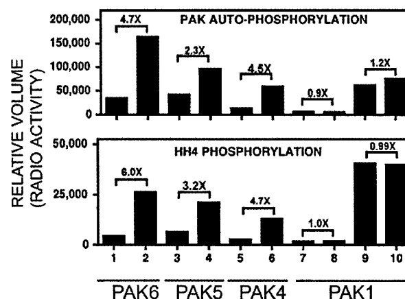
FIG. 8. Specificity of MKK6-induced PAK activation. A, sequence alignment of the activation loop region between catalytic subdomains VII and VIII of PAKs and MAP kinase family members. In both group 1 and group 2 PAKs, in addition to the previously defined autophosphorylated threonine or serine residues, a conserved TXY motif was also found within the activation loop. B, kinase activity of MKK6-modulated PAKs. 293 cells were co-transfected with MKK6(EE) and one of the following HA-tagged PAK family members: PAK1, PAK4, PAK5, or PAK6. Additionally, PAK1 was also tested by co-transfecting with a constitutive active Cdc42-V12. The kinase activity was determined by an in vitro kinase assay with anti-HA mAb immunoprecipitated kinases and analyzed by SDS-PAGE followed by autoradiography. C, Western blot demonstrated the comparable level of expression within individual PAK testing group. D, quantitation of kinase reactions from B using a PhosphorImager. The upper panel depicts levels of autophosphorylation of various PAKs. The lower panel depicts kinase activity toward histone H4. The numbers on top of each PAK group indicate fold activation in response to MKK6 co-transfection.
