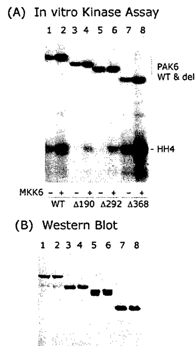
FIG. 4. Mapping PAK6 domain susceptible to MKK6-induced activation. A, 293 cells were co-transfected with MKK6(EE) and HA-tagged PAK6 WT full length and N-terminal deletion mutants Δ190, Δ292, or Δ368, respectively, for 24 h (all with N-terminal HA tags). The kinase activities of PAK6 WT, and N-terminal deletion mutants were determined by an IP kinase assay using anti-HA 12CA5 mAb. B, Western blot analysis showed equal levels of expression of PAK6 full length and deletions.
