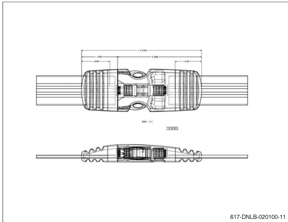
Figure 25. Schematic of redesigned buckle connector
