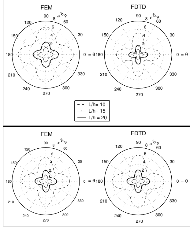
Figure 6: Polar graph of the phase error in degrees per wavelength for selected values of L/h , with \eta = 0.4 (top) and \eta = 0.01 (bottom).
