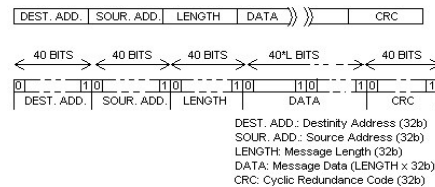
Asynchronous frame
