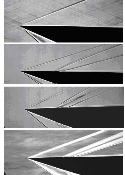
Visualizing of the boundary layer on a model ( widening of the boundary layer )
