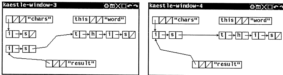
Figure 4-4: Illustration of the Validity of a Rule Using KAEStLE
