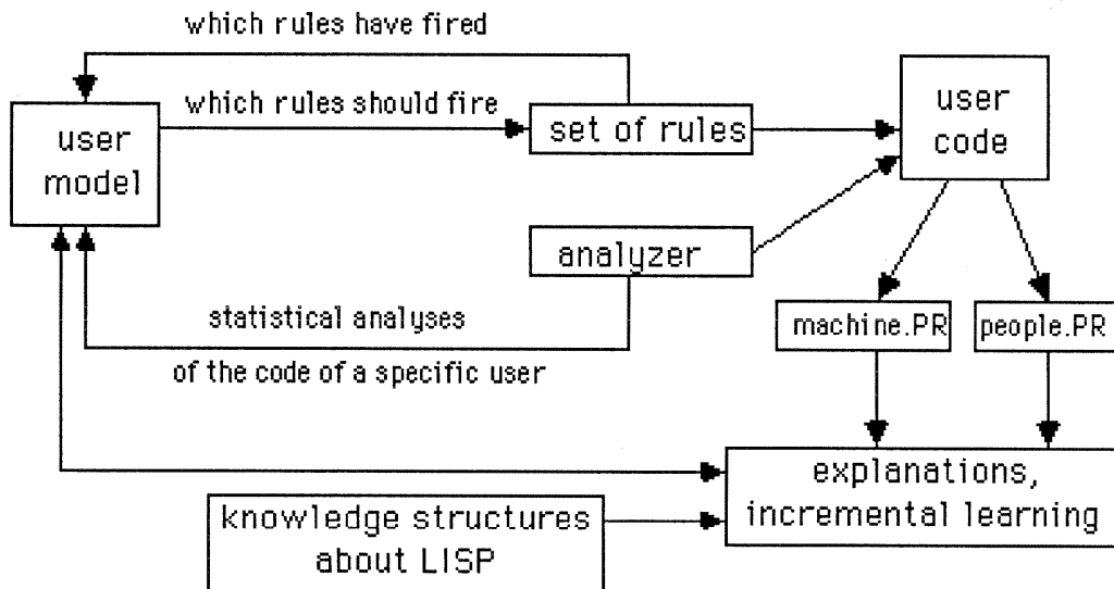
Figure 4-3: The Architecture of the LISP-CRITIC
