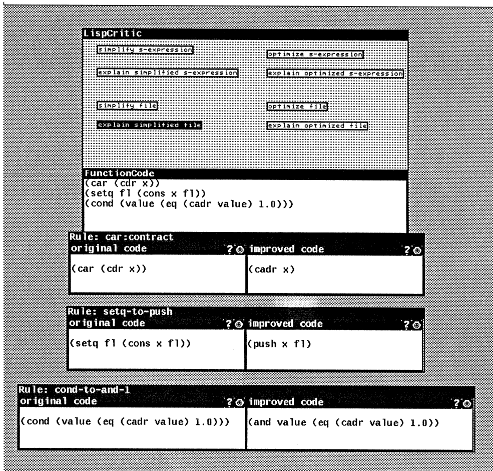
Figure 4-1: The LISP-CRITIC in Operation
