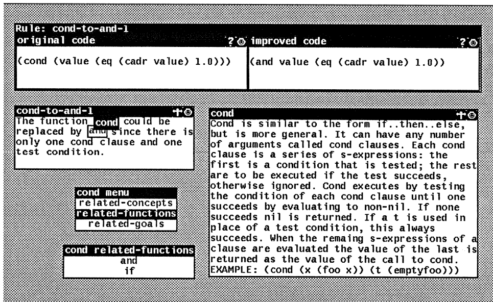
Figure 4-5: The User Browses through the Knowledge Base
