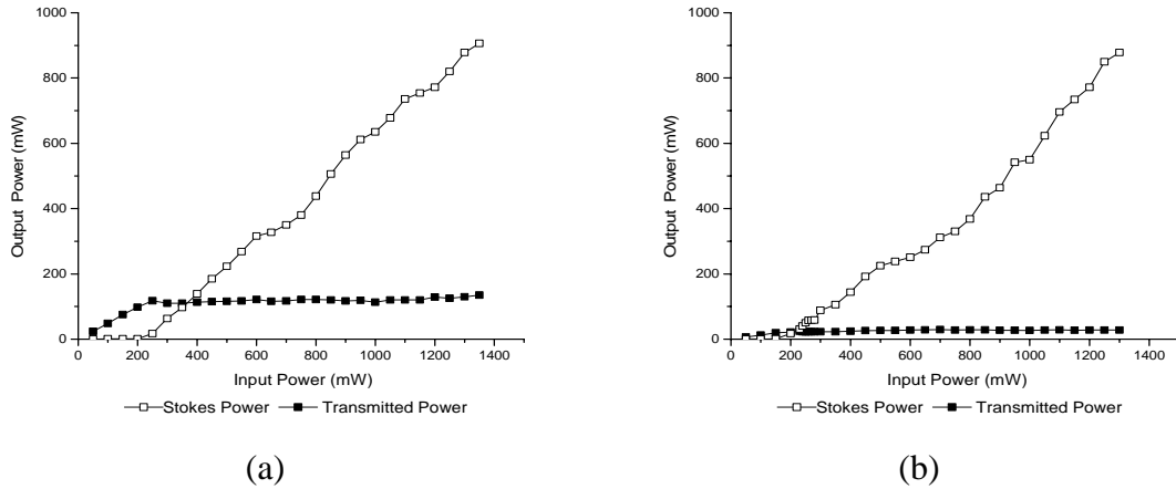
Figure 9: SBS input vs. output characteristics for (a) 2.2 km and (b) 6.6 km, 100 \mu\text{m} fibers
