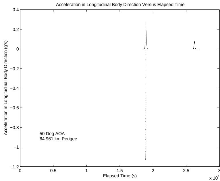
Figure 78: Acceleration in Longitudinal Body Direction Versus Elapsed Time for 50^\circ AOA, 64.916 km Perigee
