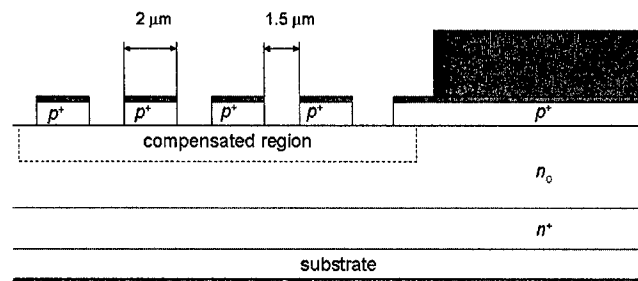
Fig. 3. Schematic cross section of a 4H-SiC FGR-structure fabricated. Dashed line represents a region where nitrogen donors are compensated by boron acceptors.
