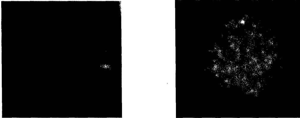
Fig. 13. Visualization of electroluminescence in a 4H-SiC p^+n DM-diode under reverse (left photo) and forward (right photo) bias.
