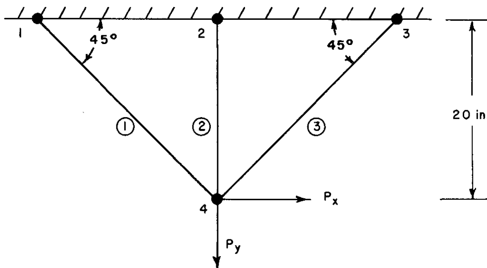
Figure 7. Three-Bar Truss
