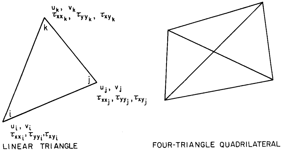
Figure 1. Four-Triangle Quadrilateral
