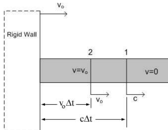
Figure 5 – Rod Impact Experiment
