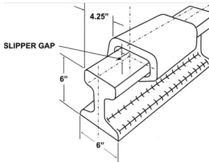
Figure 2 – Rail/Slipper Configuration
