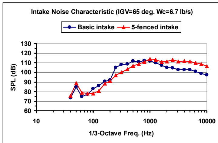
Fig.15C : Intake noise characteristic (IGV=65°, Wc=6.7 lb/s)
