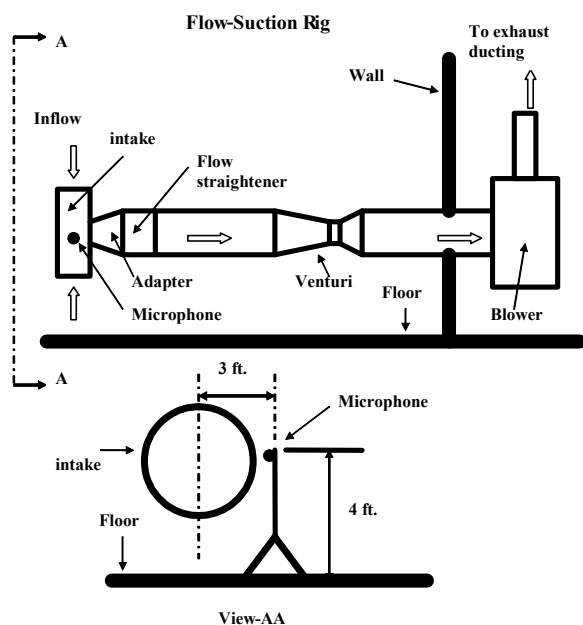
Fig.1 Test setup
