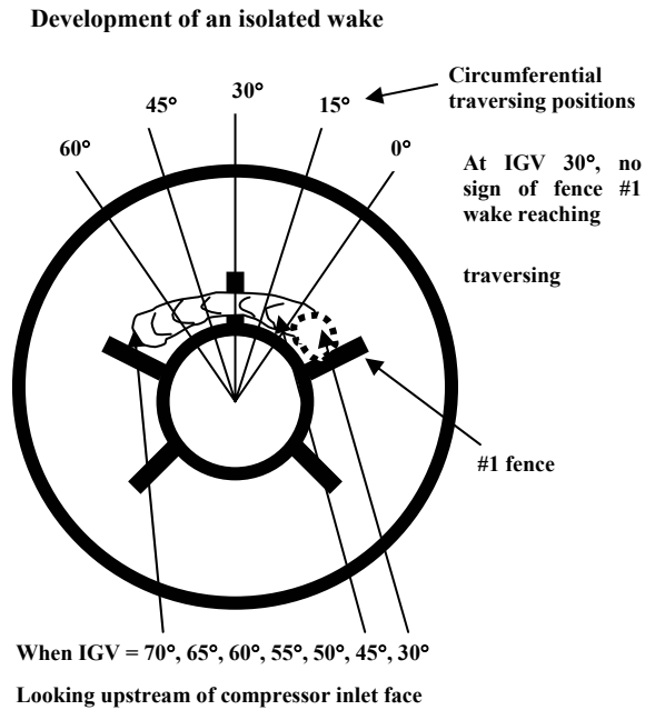
Fig.8 : Development of isolated fence-wake
