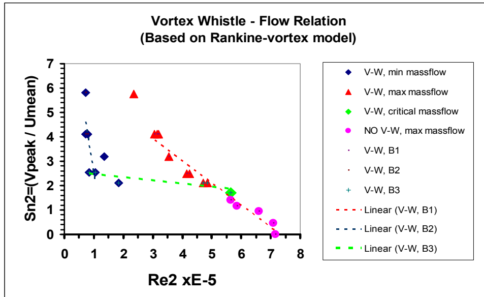
Fig.19 : Correlation for critical ratio of peak tangential to mean axial flow velocity. (B1, B2, B3 : are vortex whistle V-W boundaries #1, #2 and #3 respectively, where Re_2 = U_{mean}(R_{shroud} - R_{hub})/\nu ).
