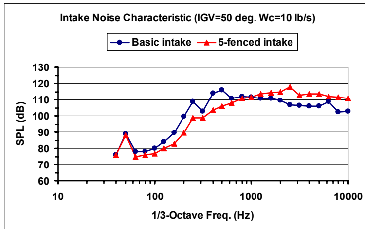
Fig.13C : Intake noise characteristic (IGV=50°, Wc=10.0 lb/s)
