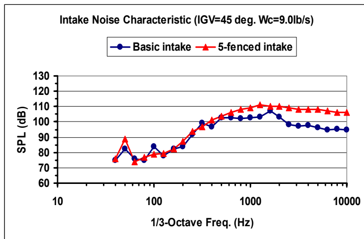
Fig.12B : Intake noise characteristic (IGV=45°, Wc=9.0 lb/s)
