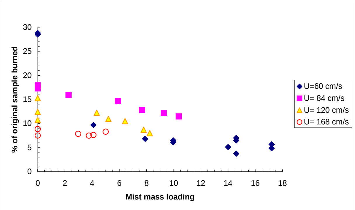
Figure 13: Fraction of the cable sample burned up to flame extinguishment versus mist mass fraction
