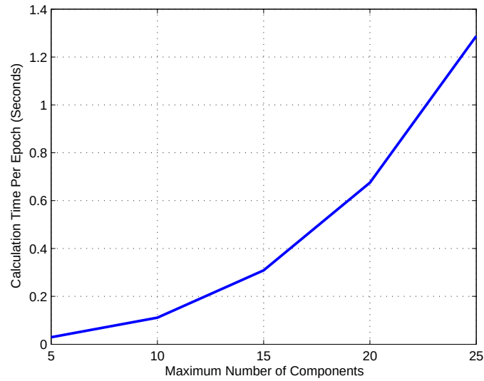
Figure 4.3: Average Calculation Time Per Epoch
