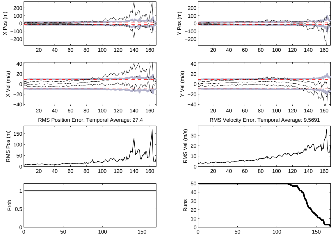
Figure 4.11: Benign Filter: Loop Model in Clutter
