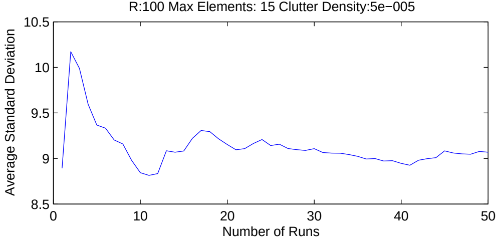
Figure 3.7: Standard Deviation vs Number of Monte Carlo Runs For Cluttered Scenario
