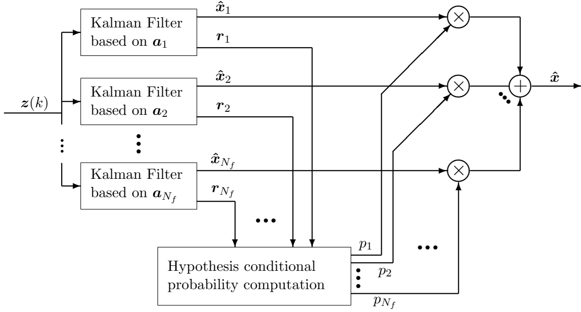
Figure 1.1: MMAE signal flow block diagram.
