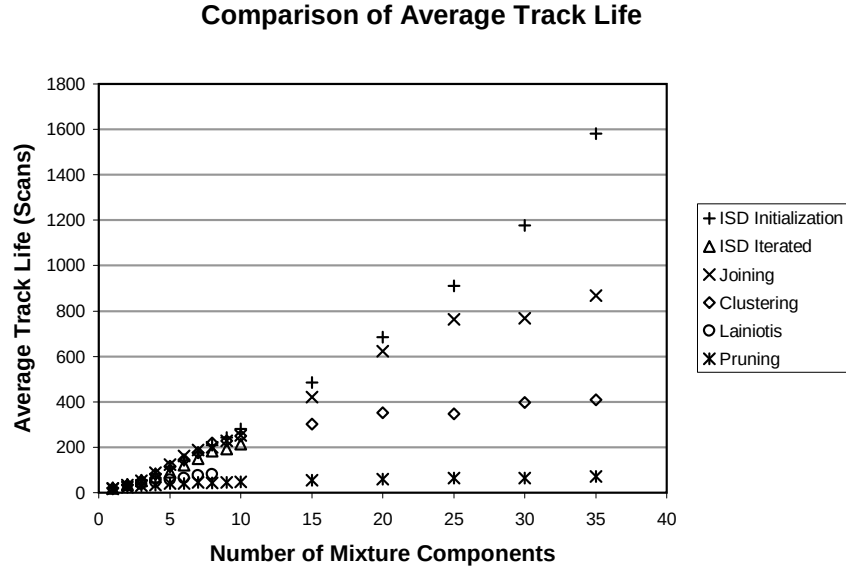
Figure 2.13: Average Track Life of Various Merging and Pruning Algorithms
