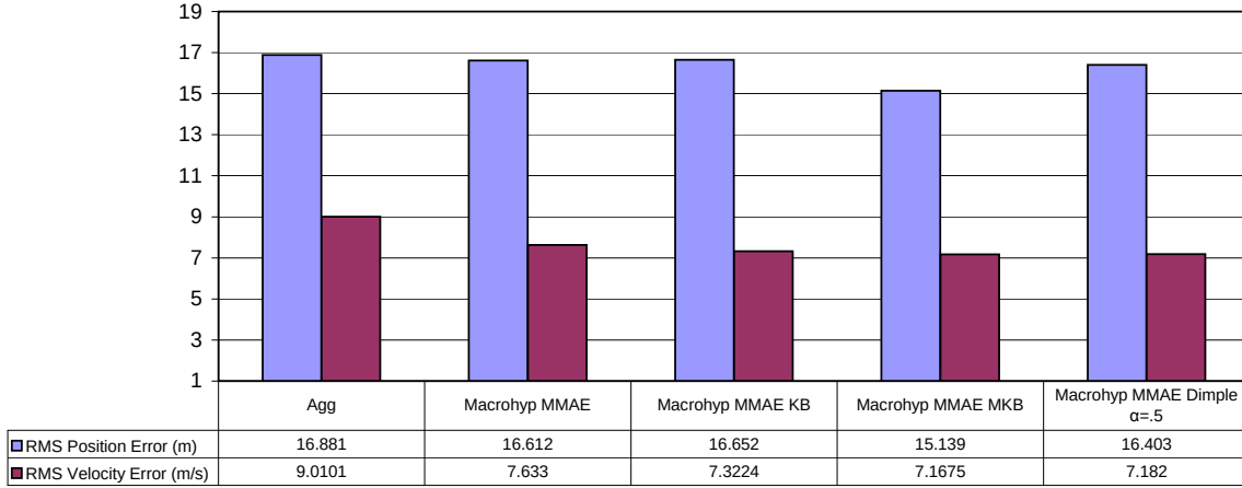
Figure 4.43: CV Broken-Loop in Clutter: Temporally Averaged RMS Values. Comparison of the standard MMAE, an MMAE using Korn & Began restarts (KB), Modified Korn & Began restarts (MKB), and the dimpled Gaussian filter.
