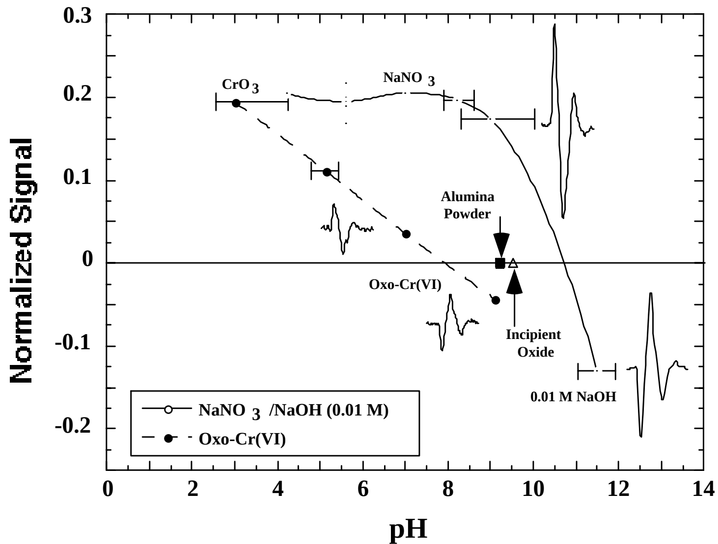
Figure 2. Relative piezo-electrokinetic response (unitless) as a function of pH for 0.01F oxo-Cr 6+ , and 0.01 M sodium nitrate or hydroxide.
