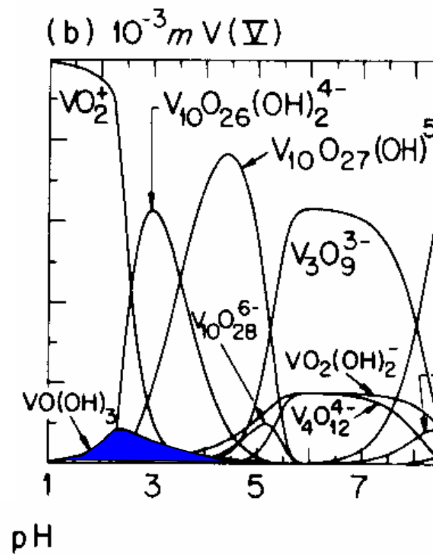
Figure 17. Equilibrium speciation of soluble V^{5+} ions in aqueous solutions at millimolar concentrations. Adapted from C.F. Baes, Jr., R. E. Mesmer, Hydrolysis of Cations , p. 210, Robert E. Krieger Publishing Co., Malabar FL (1986).
