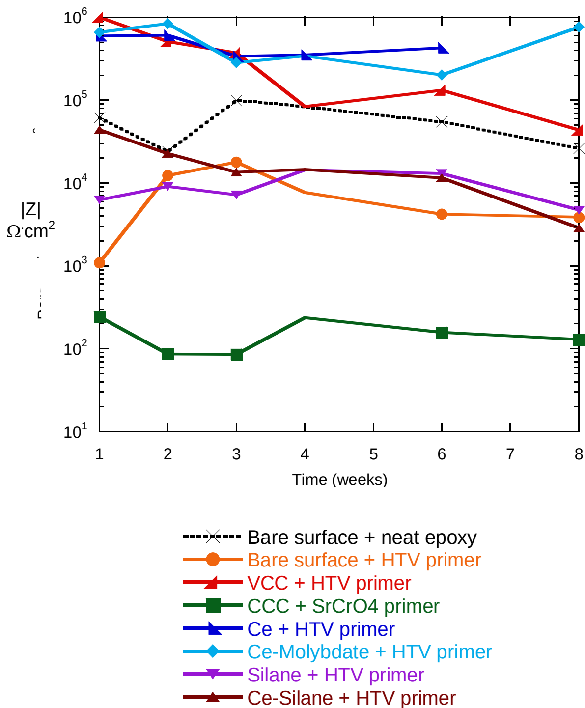
Figure 22. Variation of pore resistance, R_p , with time for salt spray tested coatings.
