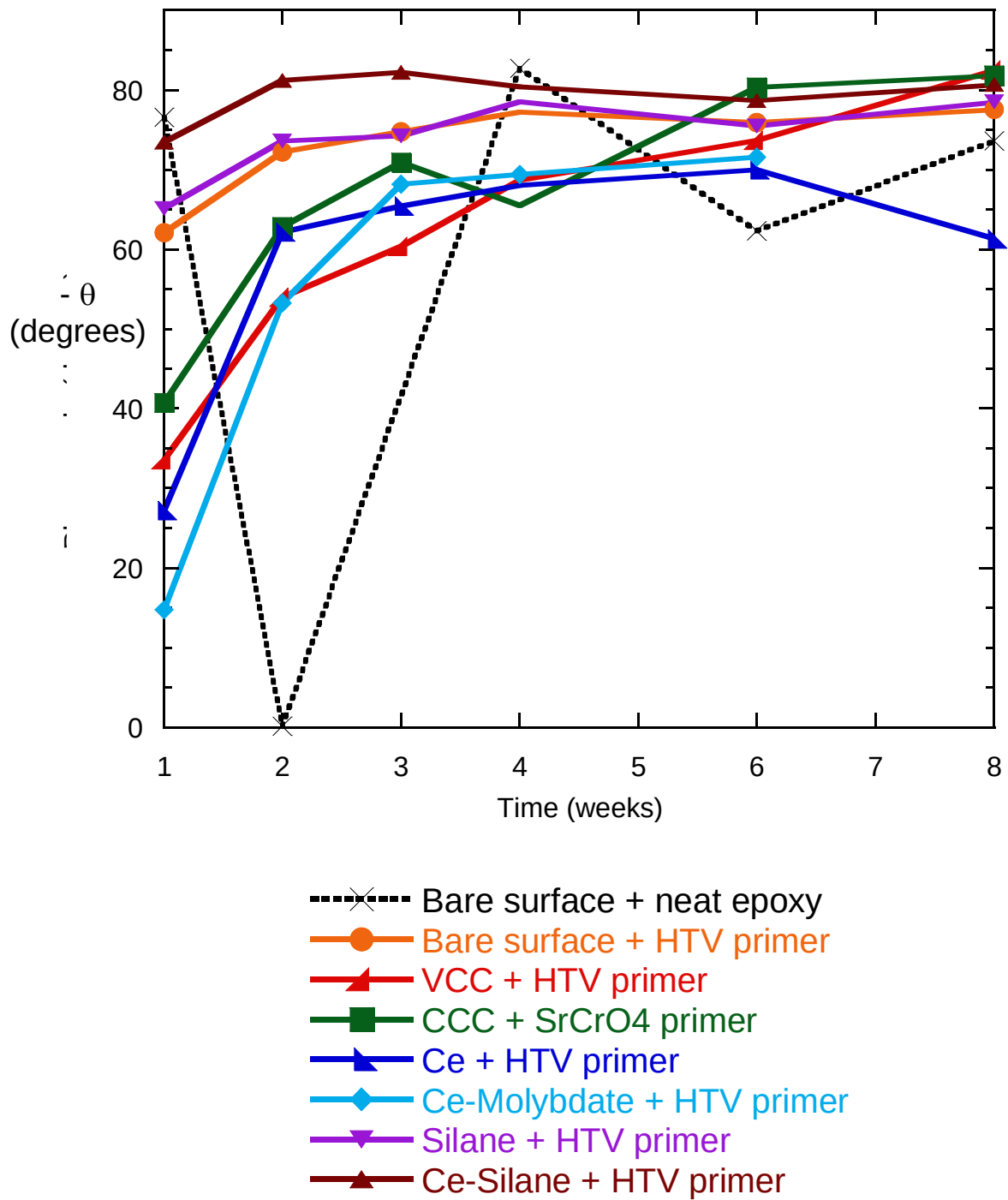
Figure 27. Variation of low frequency phase angle, -\theta , with time for UV-exposed coatings
