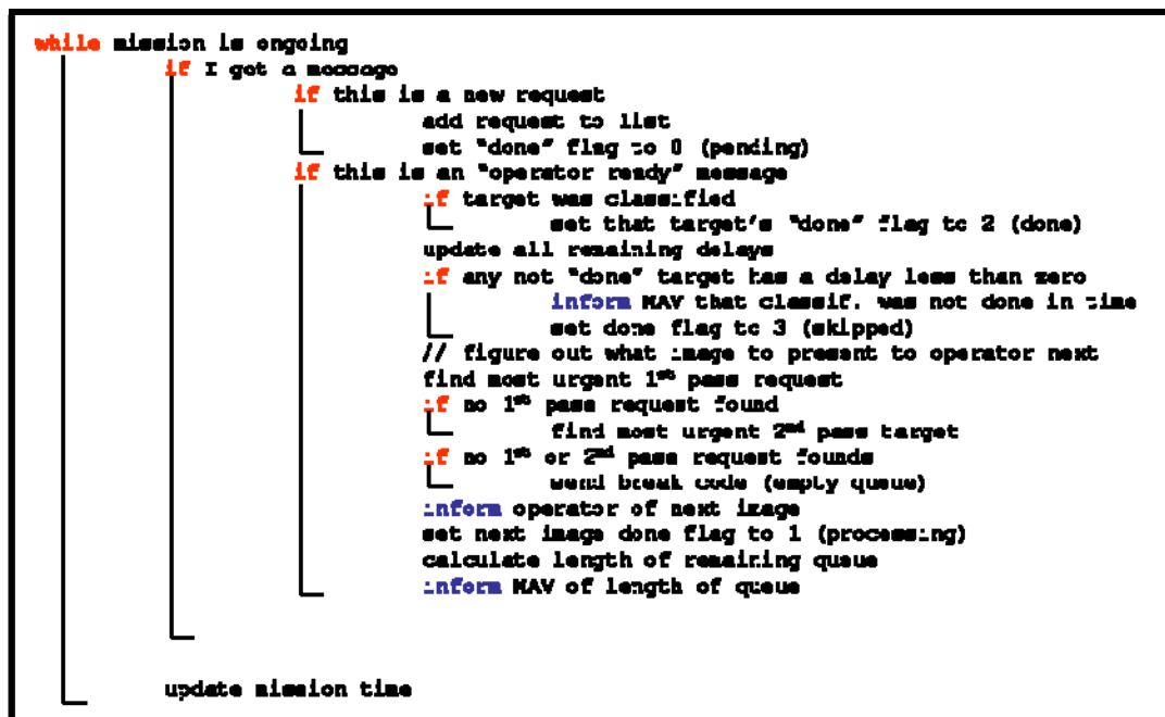
Figure 6. Scheduler pseudocode.
