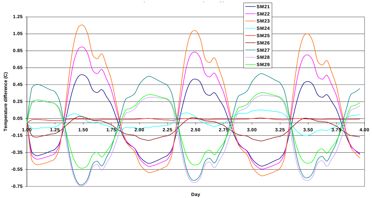
Figure 19. Differences (relative to SM standard soil) in the predicted surface temperature during the 72-hour sunny weather simulations for SM soil with Series 2 soil parameters. The curves of temperature difference group by porosity: low porosity relative to the standard soil results in daytime surface temperatures that are lower (positive temperature difference) and nighttime surface temperatures that are higher (negative temperature difference) through its effect on the soil's thermal conductivity. The thermal conductivity of the dry soil material for these experiments is 0.56 \text{ W/m}^\circ\text{C} , twenty times that of air (approximately 0.025 \text{ W/m}^\circ\text{C} ), so low porosity corresponds to relatively high soil thermal conductivity, because more of a given volume of soil is filled with soil particles rather than air. The temperature scale is changed from Figure 18 to make small temperature differences easier to distinguish.
