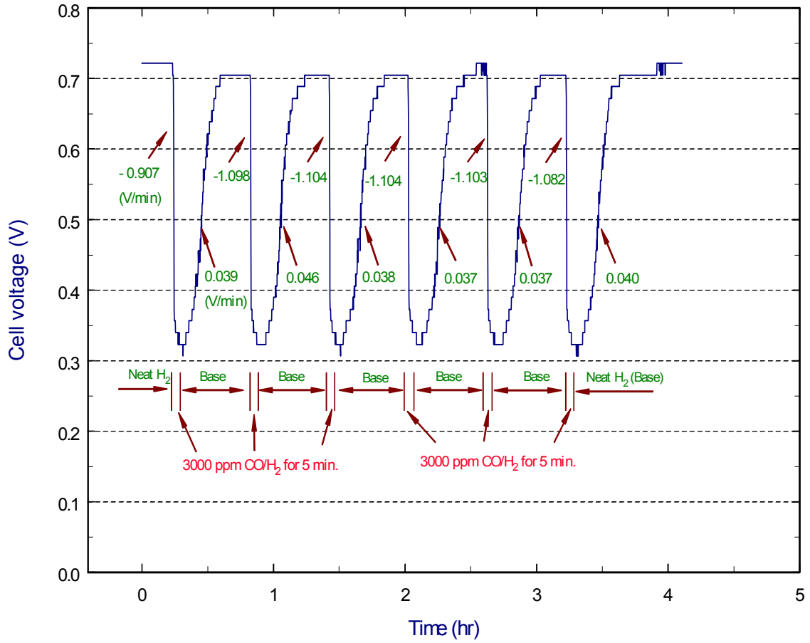
Figure 1. Transient performance with neat hydrogen and 3000 ppm CO at 600 \text{ mA/cm}^2 with CARBEL ™ CL GDM. ( T_{\text{cell}} = 70^\circ\text{C} and P(\text{A/C}) = 15/15 \text{ psig} )
