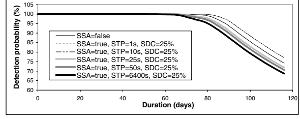
Fig. 16. Influence of sentry toggle period (STP) on detection delay (DP).
