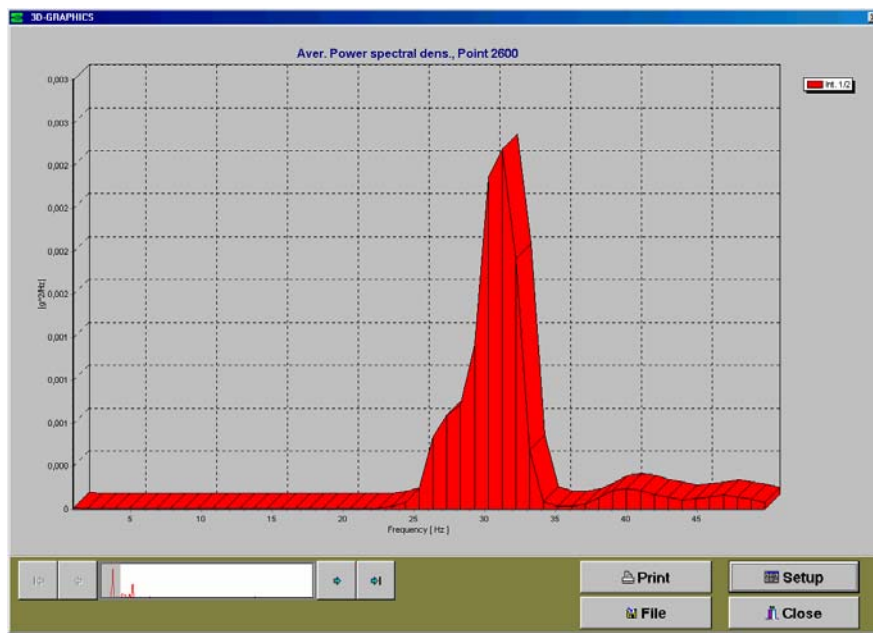
Figure 8: PSD graph of the vibration frequency, (selected region of 1st interval) Z axis.
