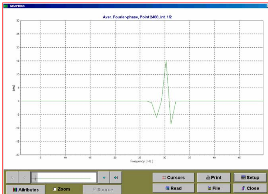
Figure 9: The interval Fourier phase graph, (selected region) Z axis.
