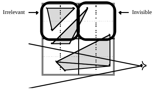
Figure 8: Invisible nodes are completely outside the view frustum. Irrelevant nodes are invisible and contain no vertices of visible triangles.
