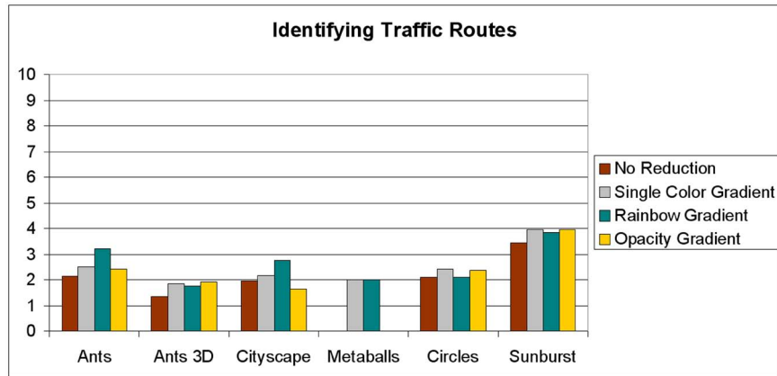
Figure 26: Task-Based Evaluation: Identifying traffic routes.
