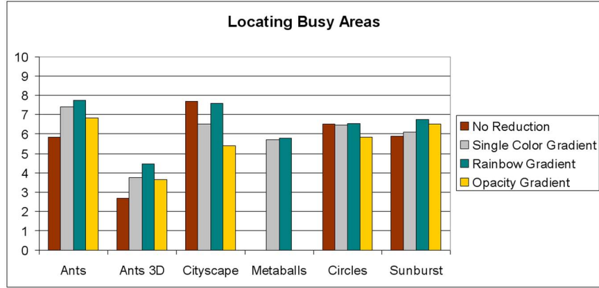
Figure 25: Task-Based Evaluation: Locating busy areas.
