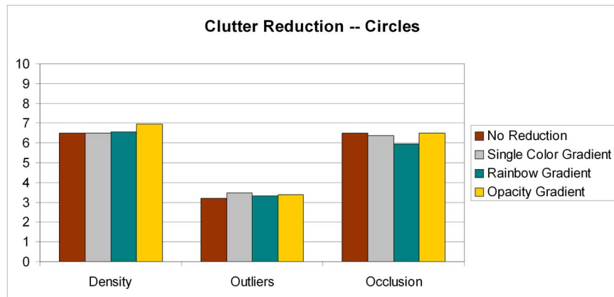
Figure 23: Circles: Effectiveness of clutter reduction.
