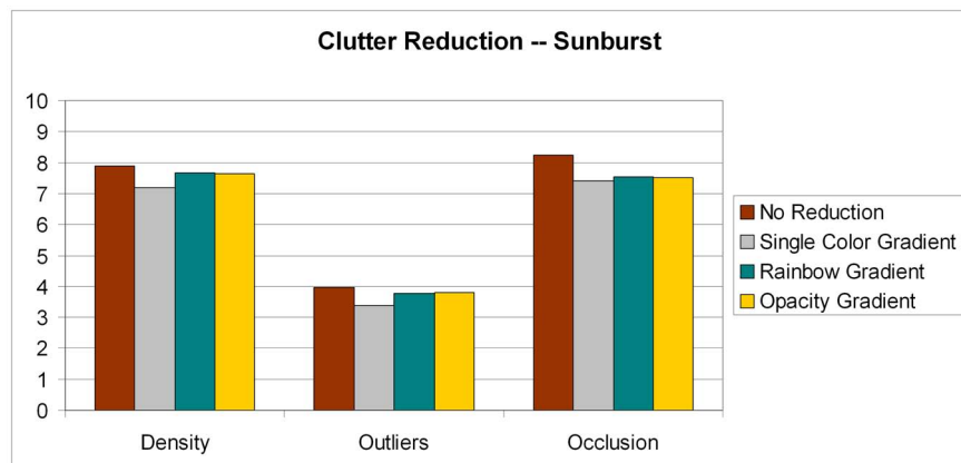
Figure 24: Sunburst: Effectiveness of clutter reduction.
