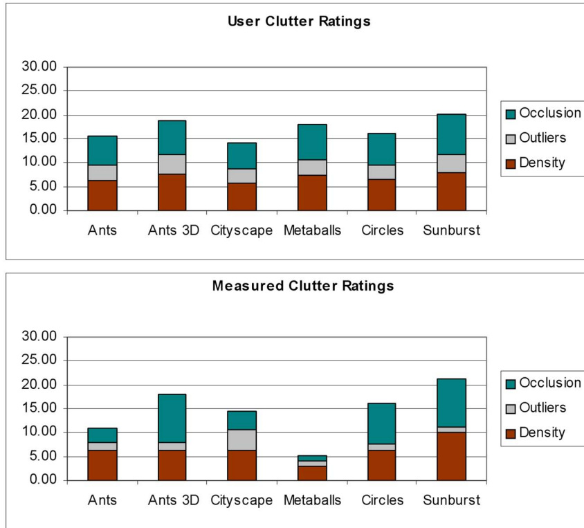
Figure 15: Amount of clutter present in all visualizations.
