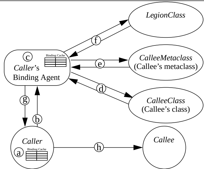
FIGURE 9. Potential steps in the Legion binding and class-of mechanisms—Caller must bind the LOID of Callee to an OA for low-level communication. Caller may already have a cached binding for Callee (a), or may need to consult a binding agent (b). The binding agent may have a cached binding for Callee (c), or may need to consult Callee’s class, CalleeClass , for the binding (d). In order to communicate with CalleeClass , the binding agent needs a binding for CalleeClass . If the binding agent does not have CalleeClass ’s binding, it may need to consult CalleeClass ’s metaclass (e). If the binding agent does not know the binding for this metaclass, the process repeats itself. The recursion is guaranteed to terminate at the root of the binding tree, LegionClass (f). Eventually, the binding agent returns Callee’s binding (g) and Caller can send messages directly to Callee (h).
